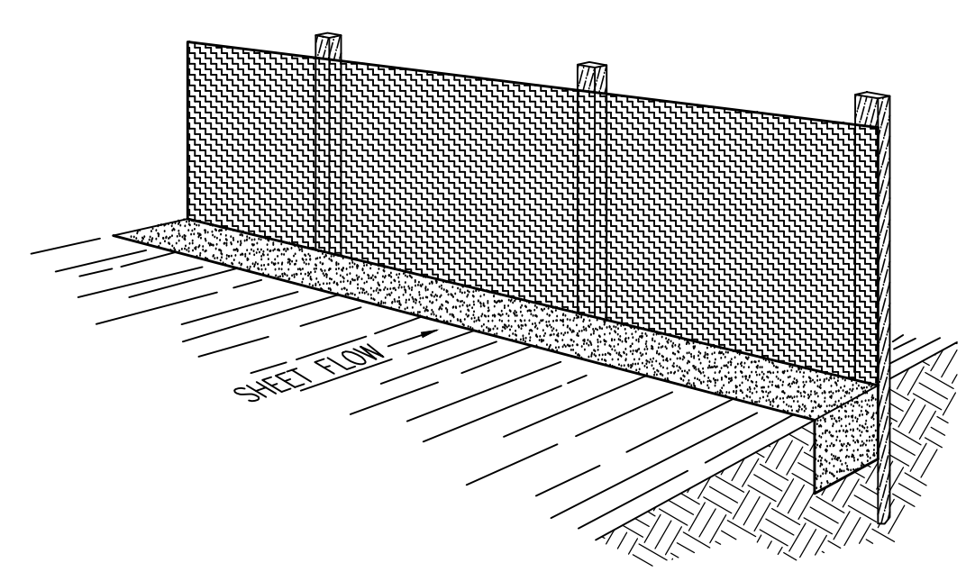
Perspective View
