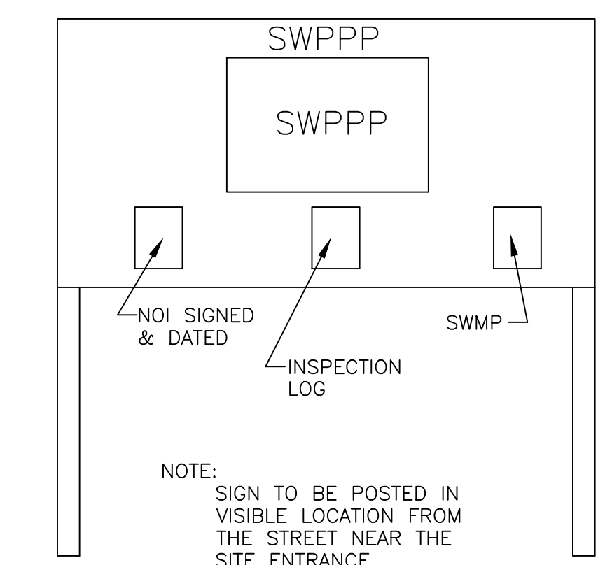
Sample SWPPP Board (4'x8' Sheet of Plywood)
