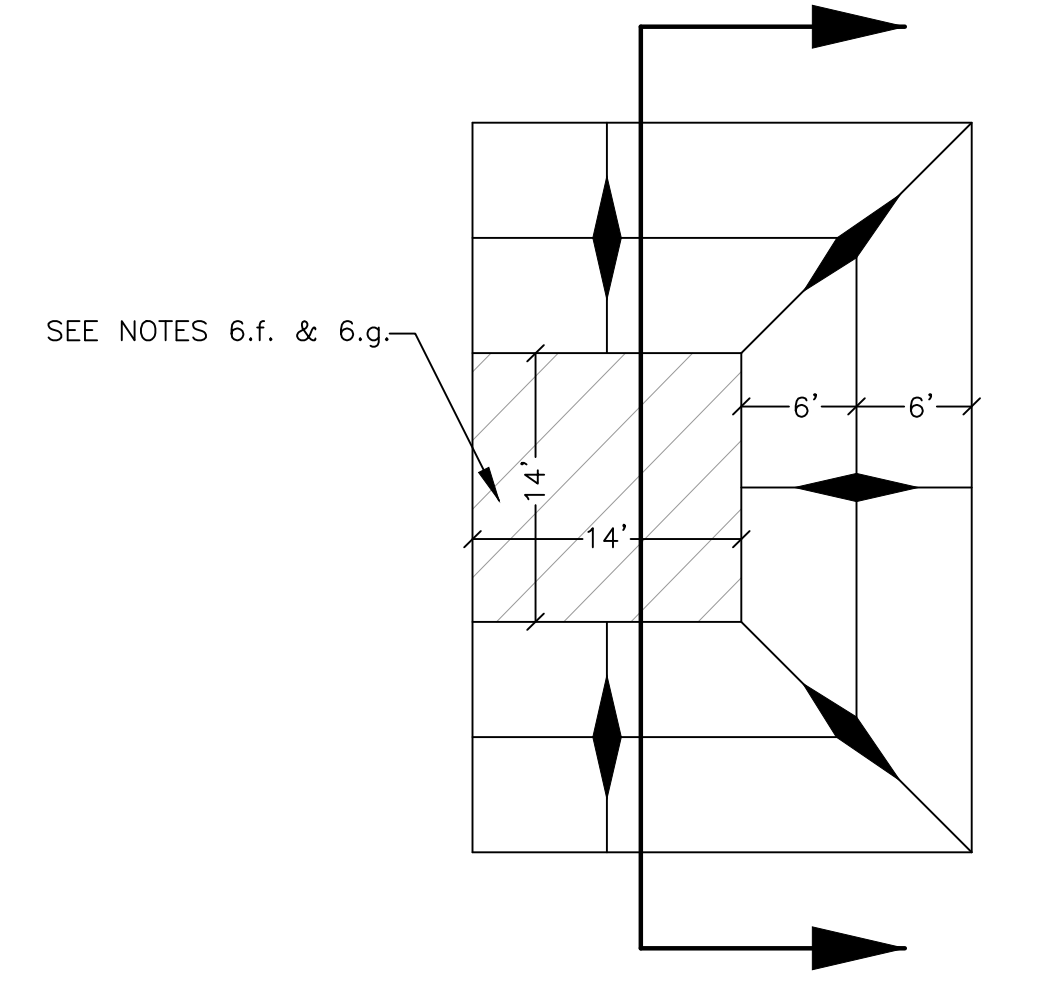
Concrete Washout Area w/ 10 mil Plastic Liner
