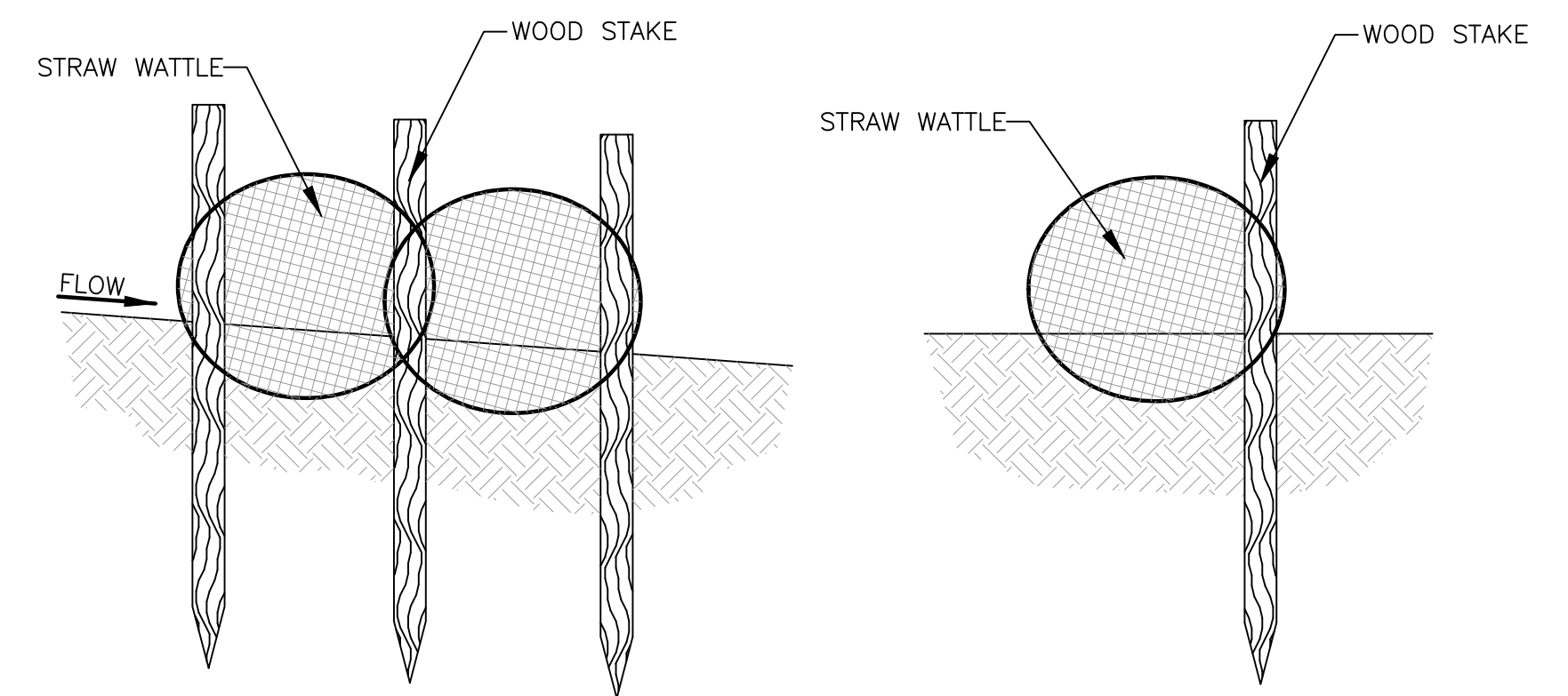
Stake Detail
