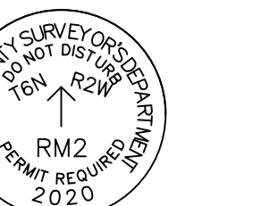
MONUMENT DETAIL 6 (NOT TO SCALE)
