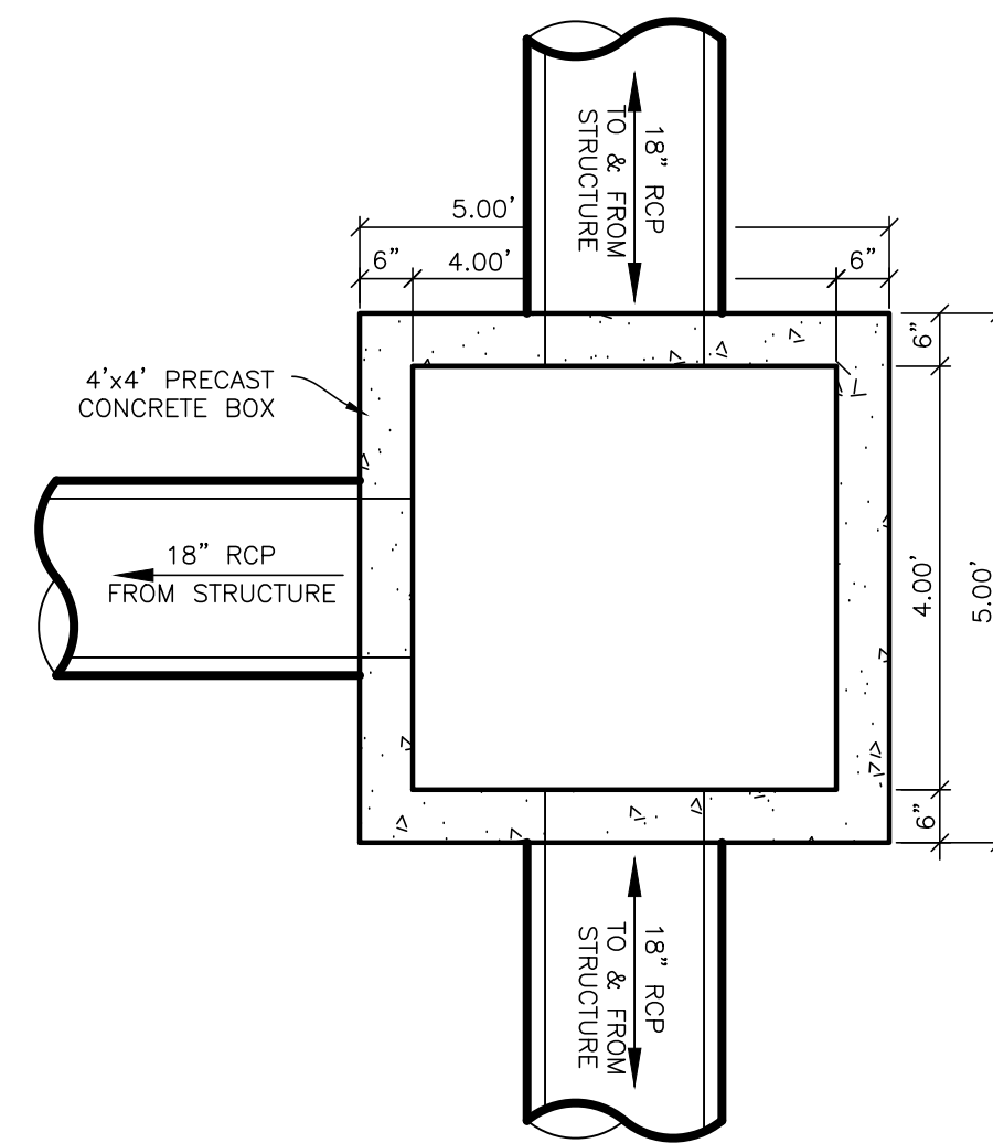
Irrigation Box Detail SCALE: NONE
