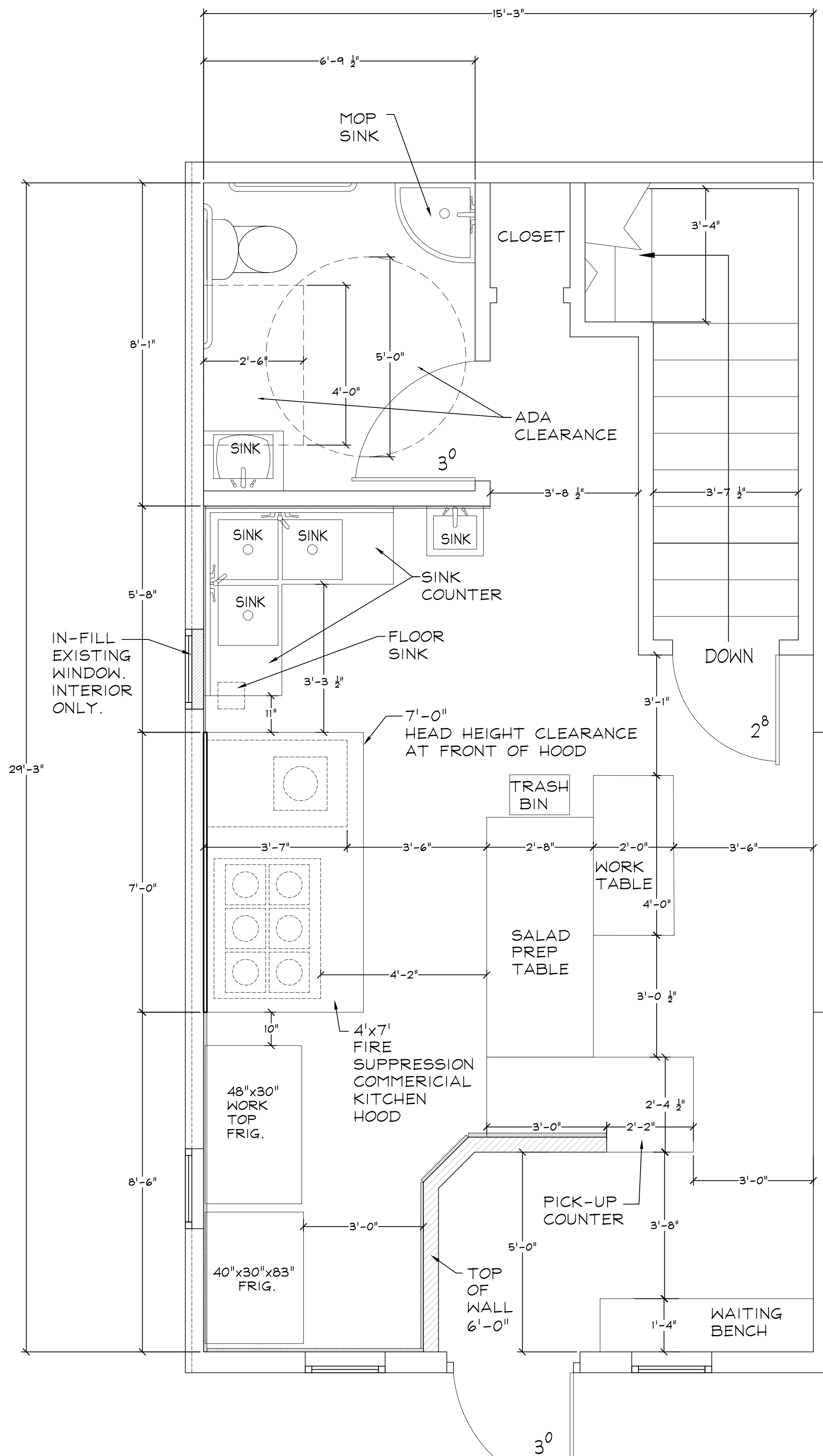
SAWASDEE THAI MAIN LEVEL RETROFIT PLAN SCALE: 1/2" = 1'-0"
