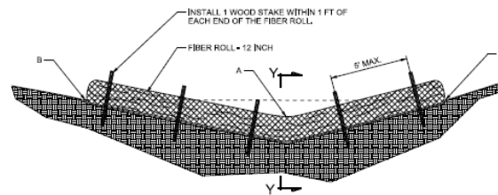
ELEVATION CHECK DAM - FIBER ROLL
