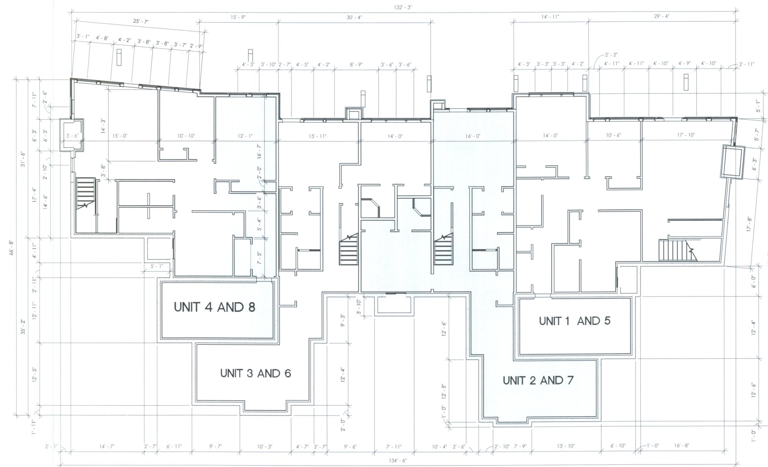
LOWER LEVEL FLOOR PLAN
