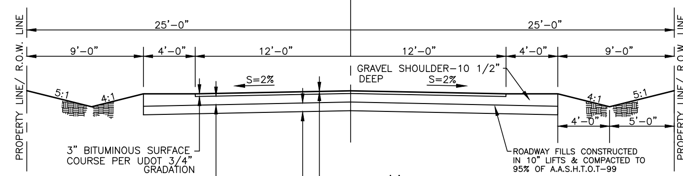
Street Section (50' R.O.W.)
