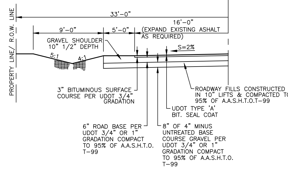
1300 South Street Section
