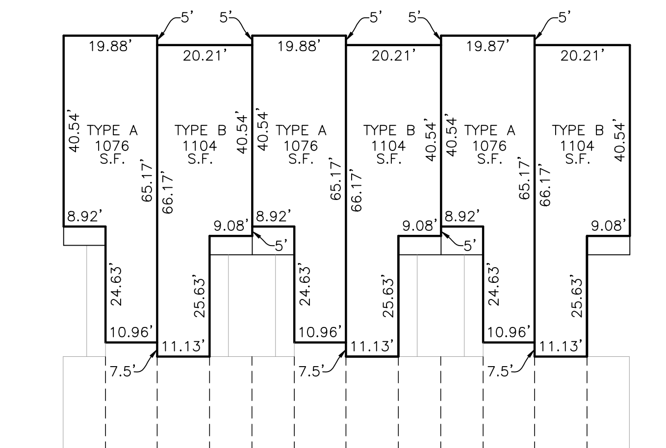
TYPICAL UNIT DETAIL NOT TO SCALE
