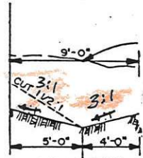
DETAIL DRAINAGE SWALE
