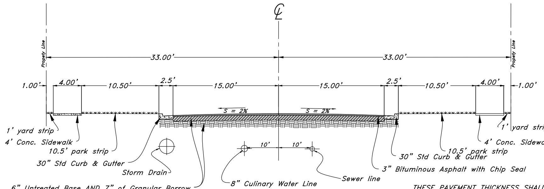
Standard Rural Roadway Section
