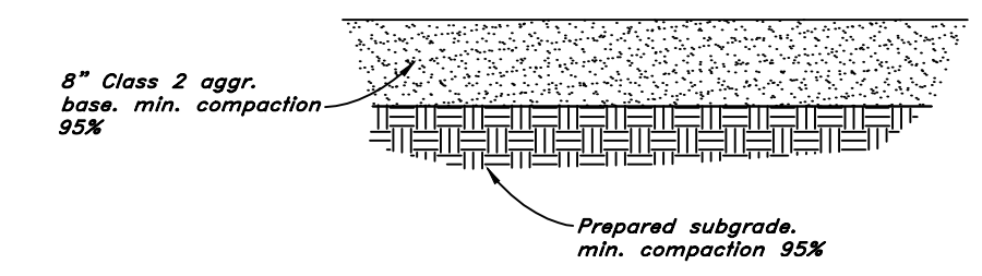
GRAVEL DRIVE DETAIL
