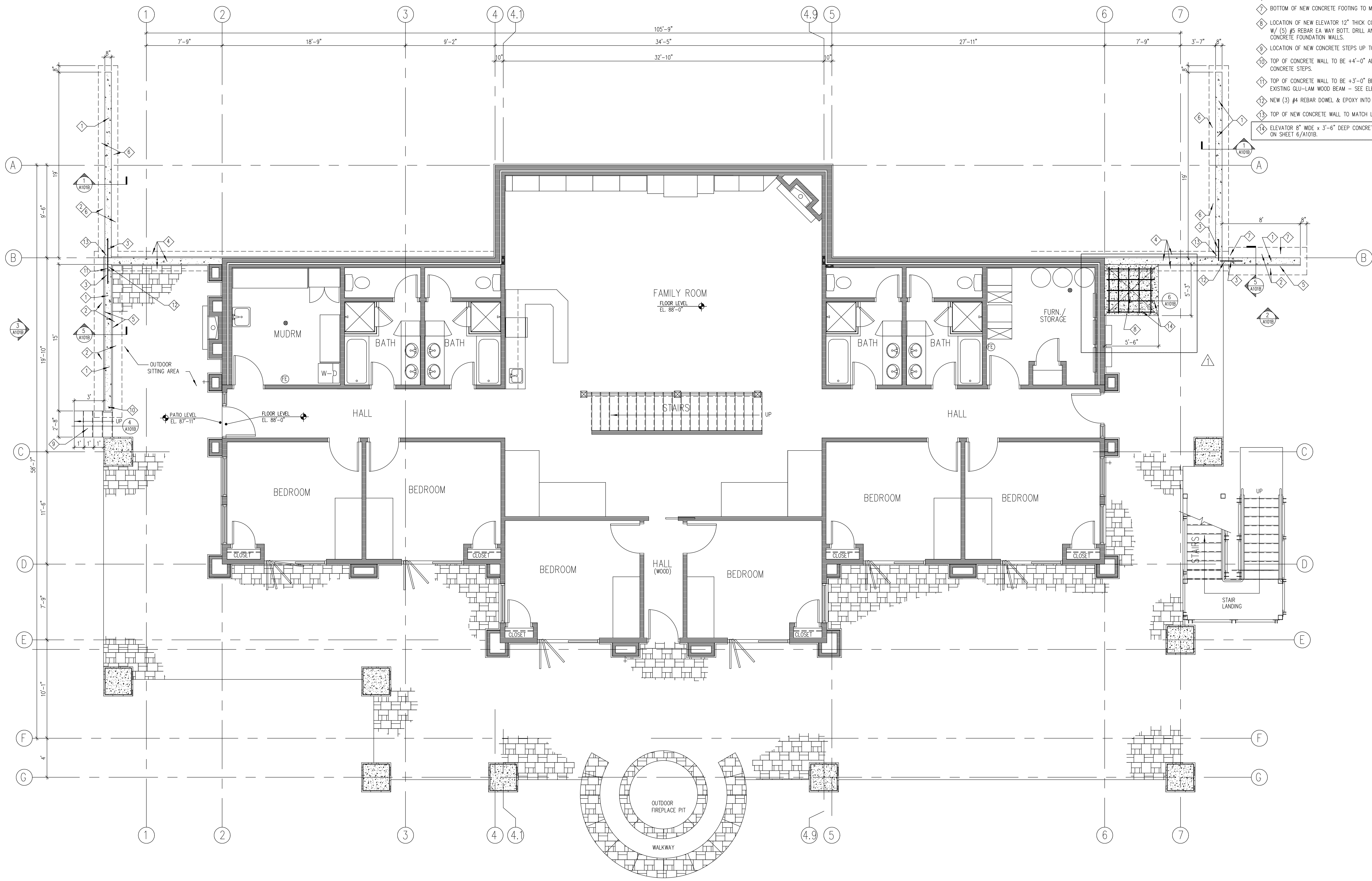
1 LOWER FLOOR PLAN CONCRETE RETAINING WALLS A101A SCALE: 1/4" = 1'-0"
