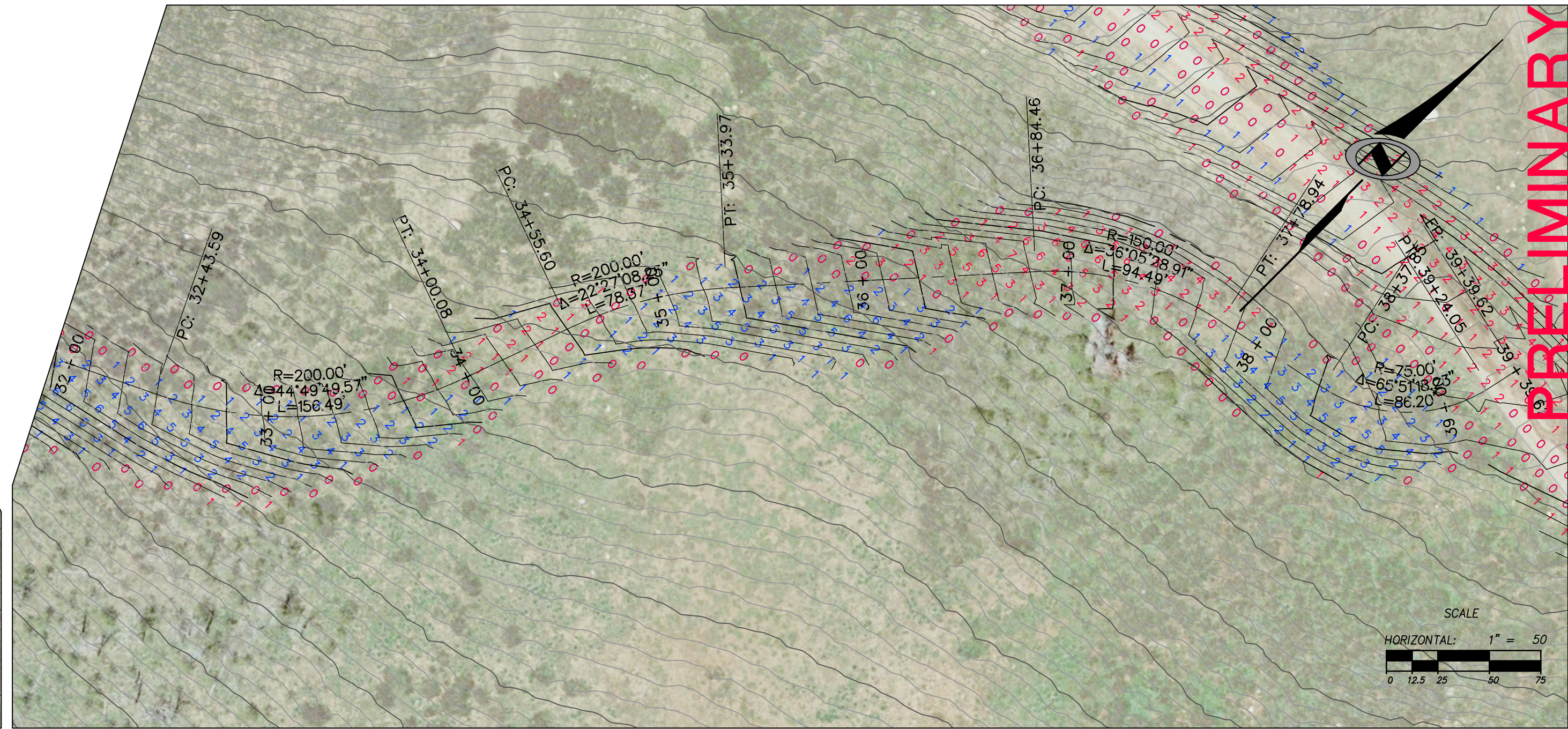
PROPOSED PH1 RD08 STA: 25+00.00 TO 39+39.62
