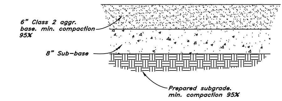
GRAVEL DRIVE DETAIL
