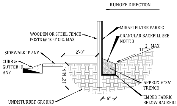
B TEMPORARY SILT FENCE SCALE: NONE
