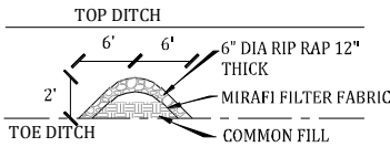
B-B' SECTION
