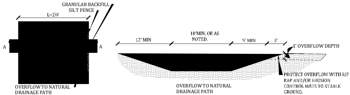
PLAN VIEW
