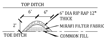
B-B' SECTION
