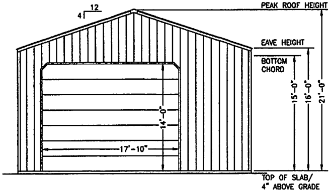
GABLE END ELEVATION - WEST
