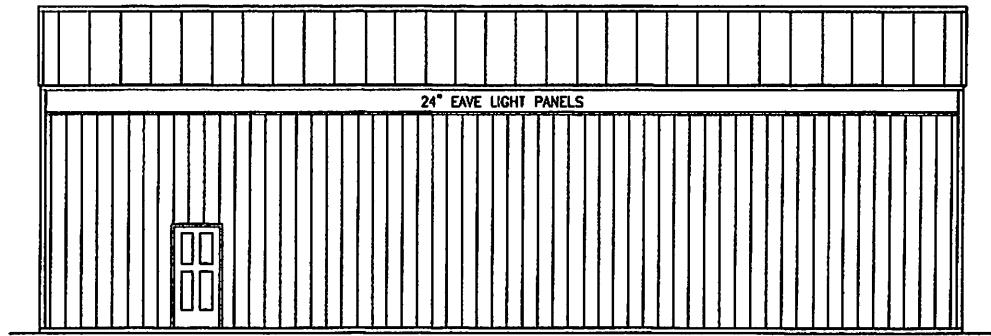
SIDE ELEVATION - NORTH
