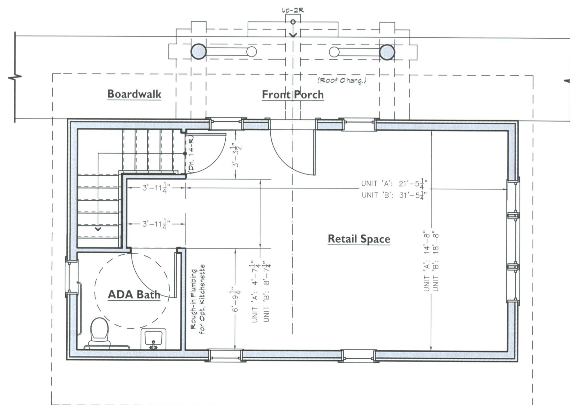
1 First Floor Plan - Side Entry (Log Veneer)
