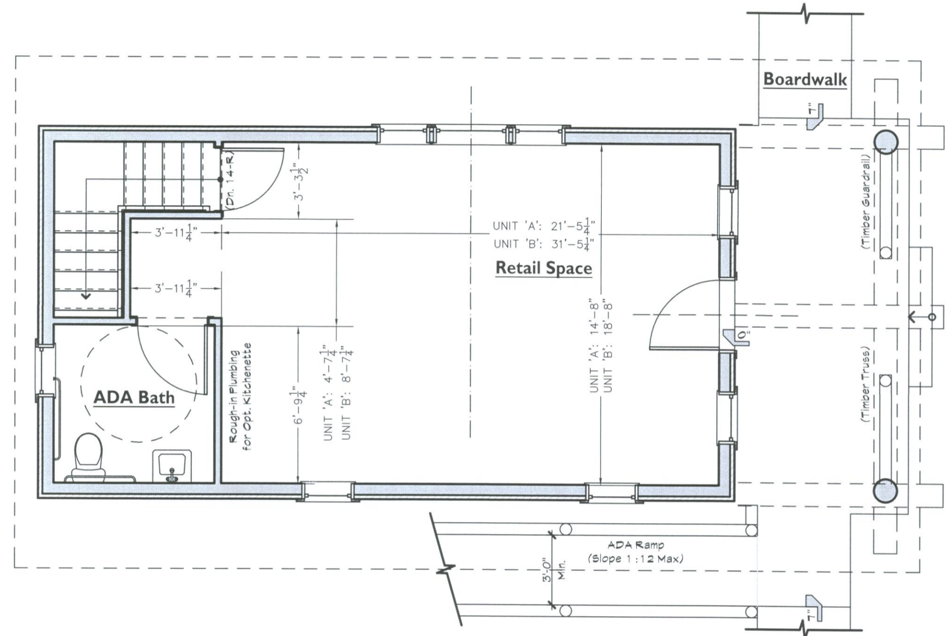
1 First Floor Plan - Front Entry (Log Veneer)
