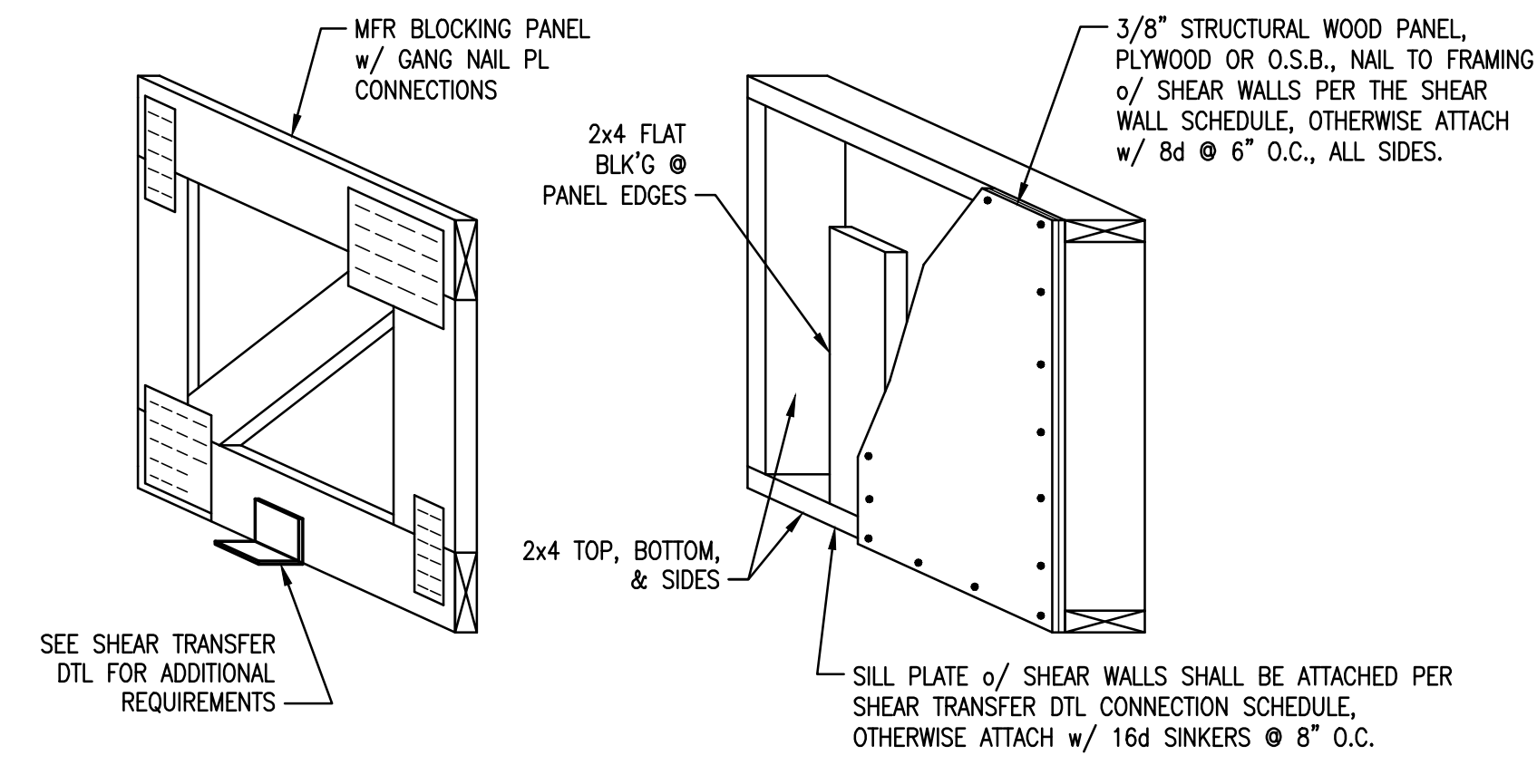
TYPICAL BLOCKING PANEL
