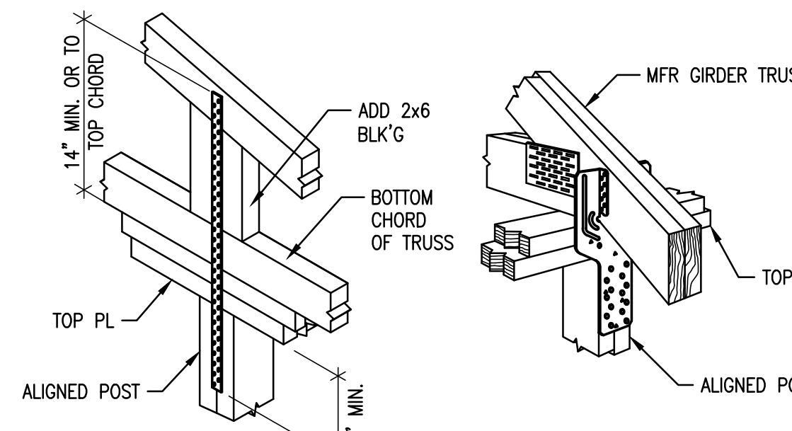
TYPICAL LGT2 INSTALLATION
