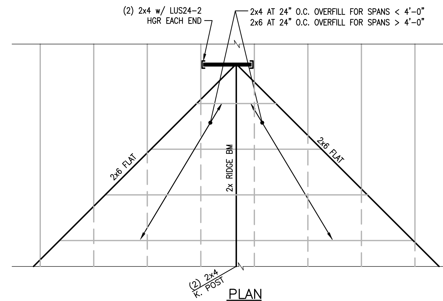
TYPICAL OVERBUILD
