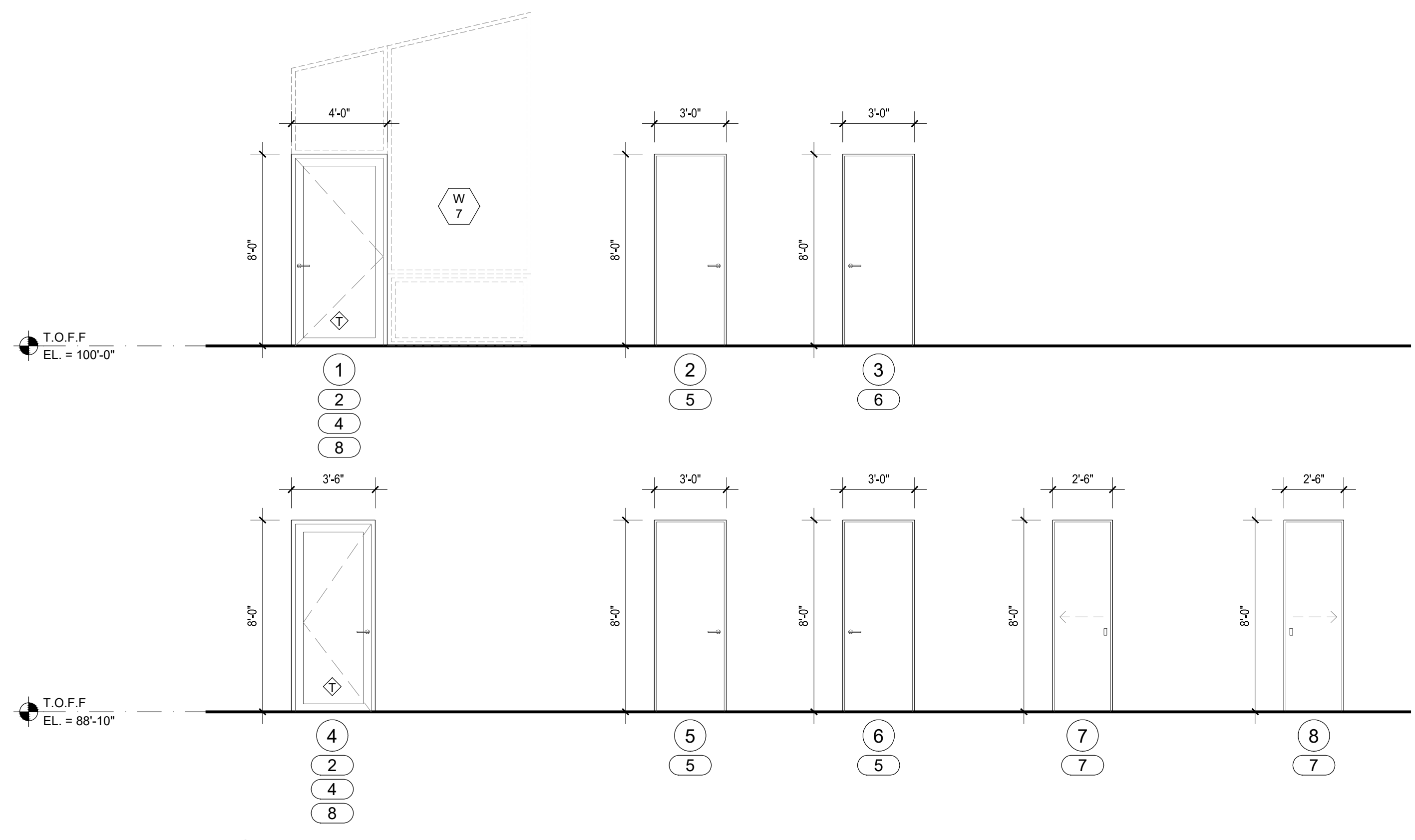
B Door Schedule SCALE 1/4" = 1'-0"
