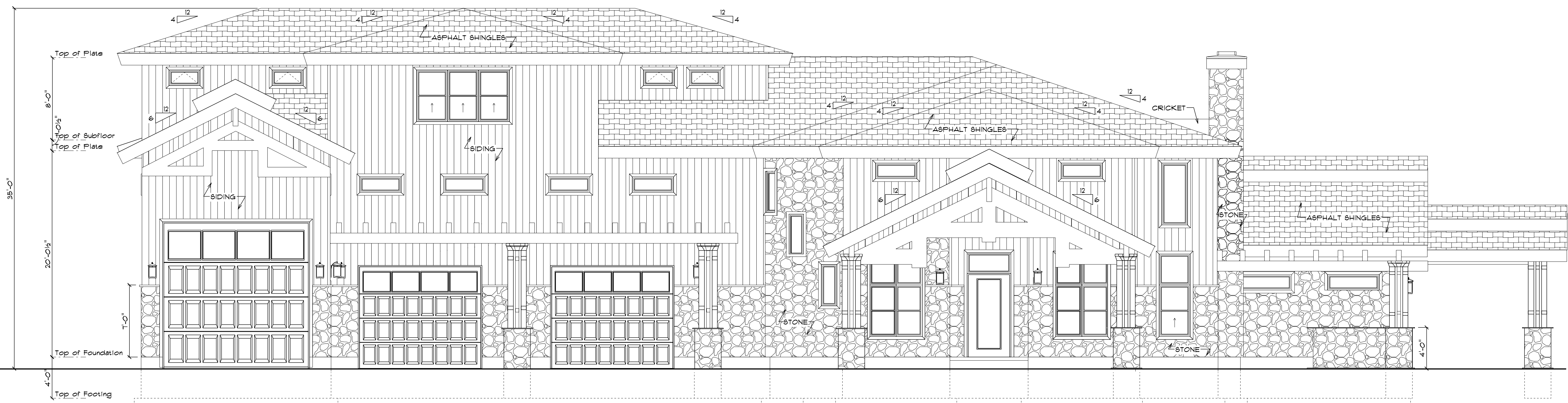
Front SCALE: 3/16" = 1'-0"
