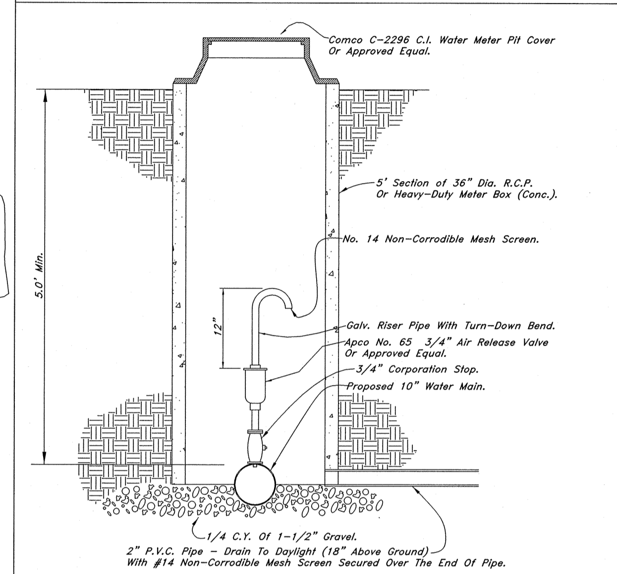
5 Air Release Detail Not to Scale
