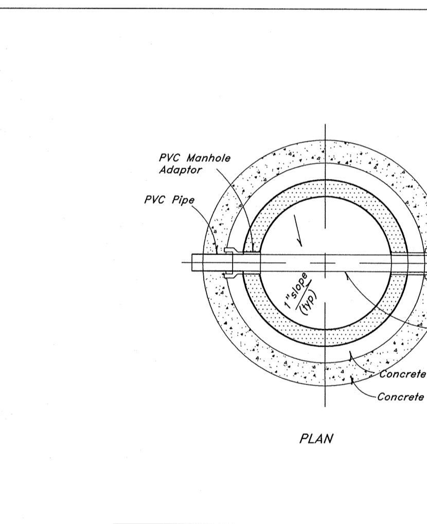
8 Typical 4.0' Manhole Detail Not to Scale
