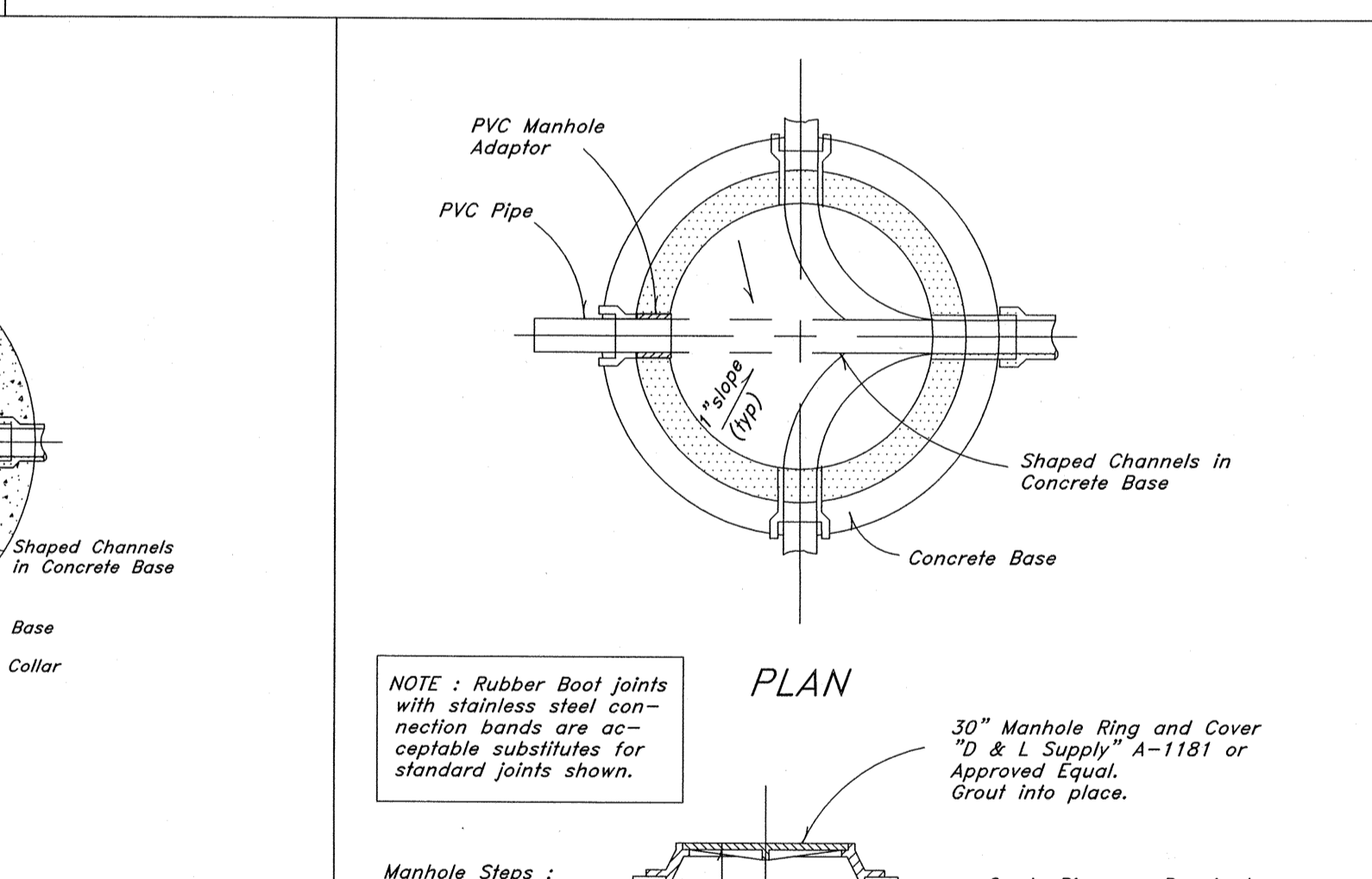
9 Typical 5.0' Manhole Detail Not to Scale
