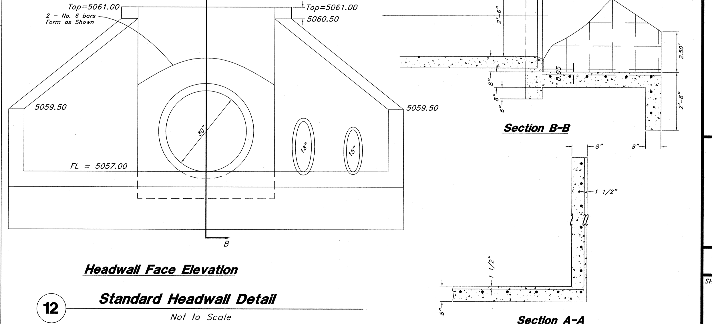
Inlet Headwall
