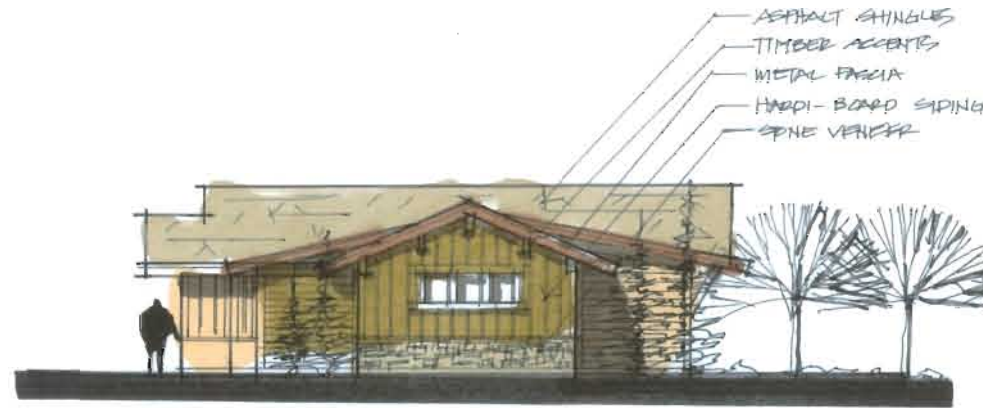
NORTH ELEVATION CONDO (EAST) GARAGE
