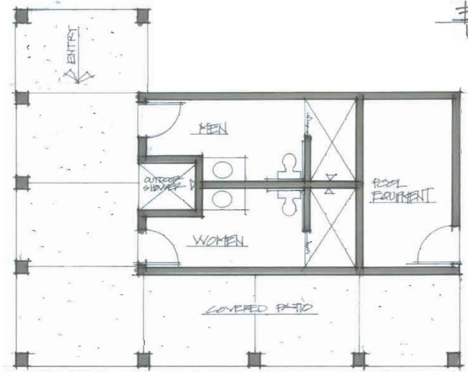
POOLHOUSE FLOOR PLAN 1/4" = 1'-0"
