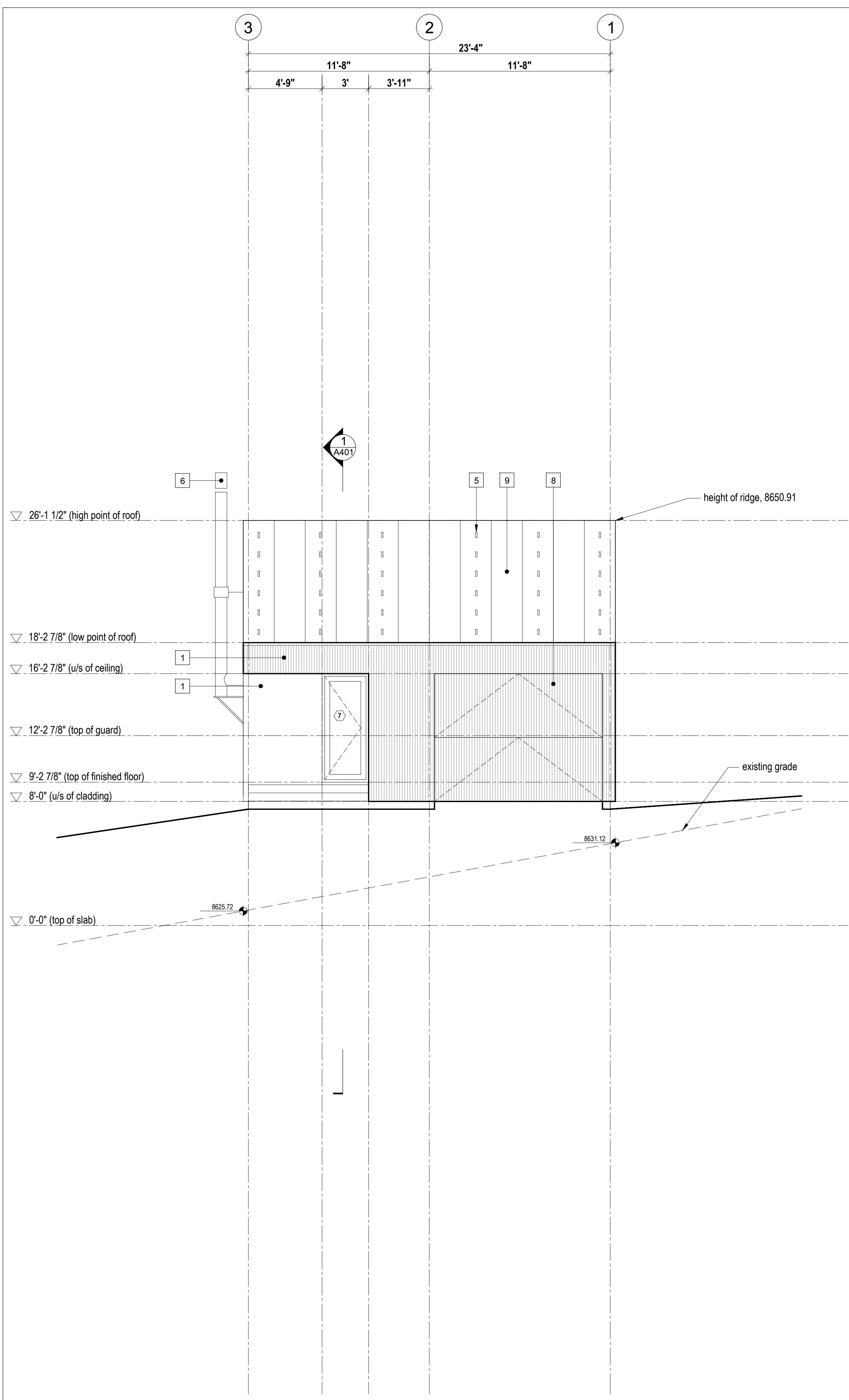
2 West Elevation Scale 1/4" = 1'-0"
