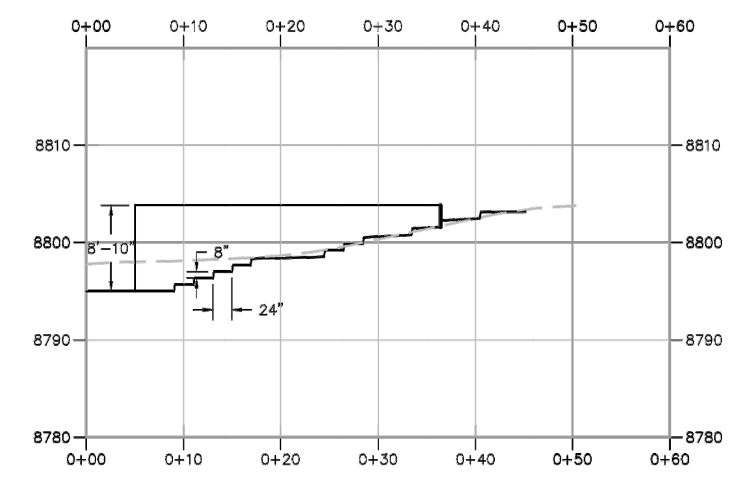
STAIR PROFILE
