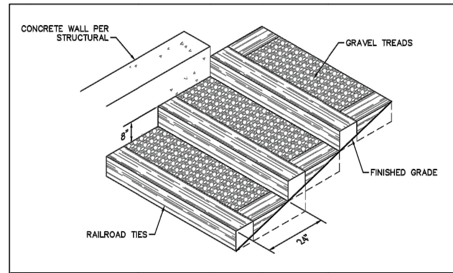
STAIR DETAIL
