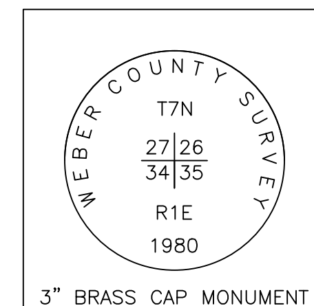
Monument Detail 2 (NOT TO SCALE)
