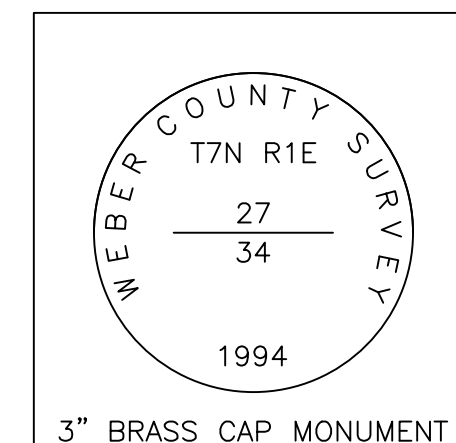
Monument Detail 1 (NOT TO SCALE)
