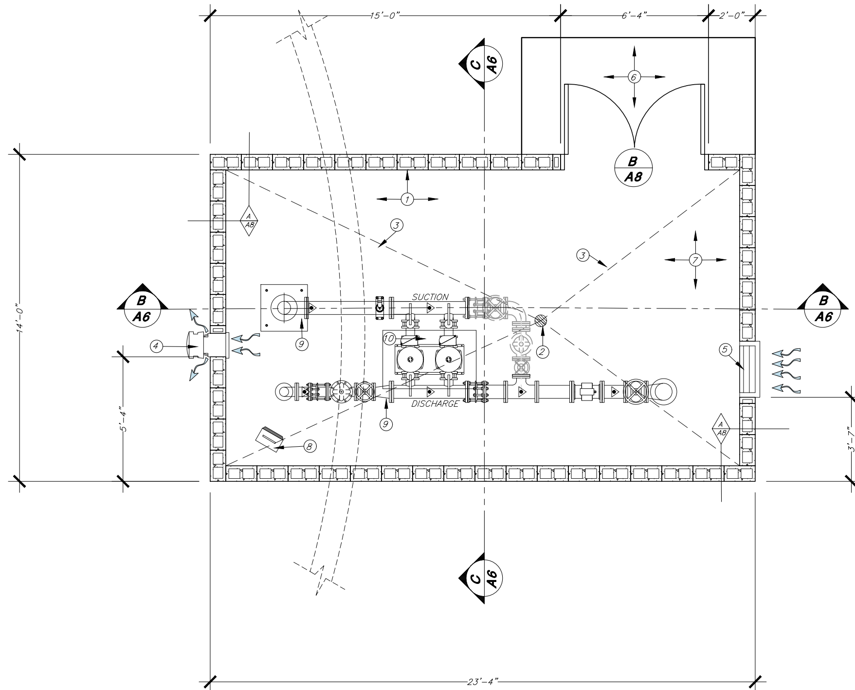
FLOOR PLAN SCALE: 1"=4'
