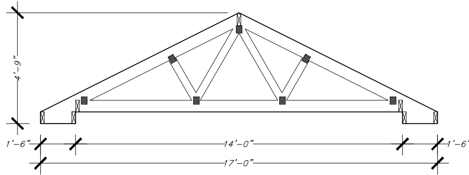
FRAME TYPE A
