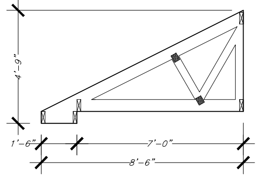
FRAME TYPE B
