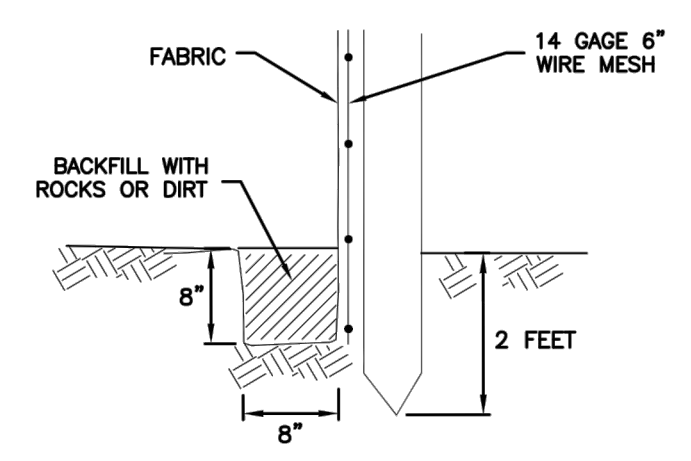
TOE DETAIL
