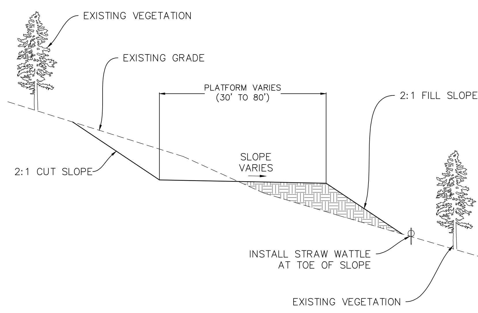
SKI TRAIL - TYPICAL CROSS SECTION
