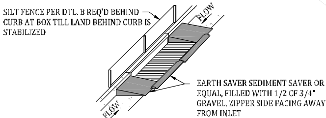
SANDBAG OPTION
