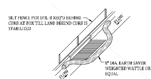
WATTLE OPTION
