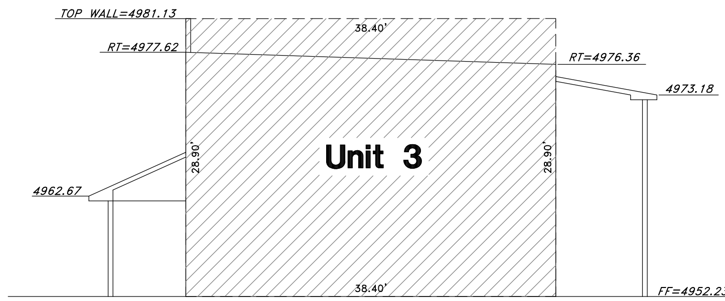
Section C-C
