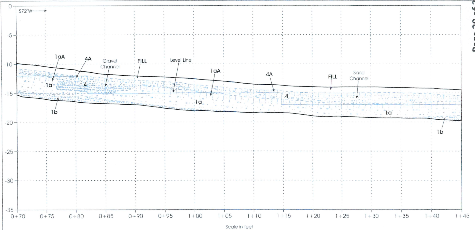
TRENCH 1 LOG, SHEET 2 SURFACE FAULT RUPTURE HAZARD EVALUATION Cedar Cove Subdivision Lot 28-A 6696 South 2850 East Weber County, Utah FIGURE 4B
