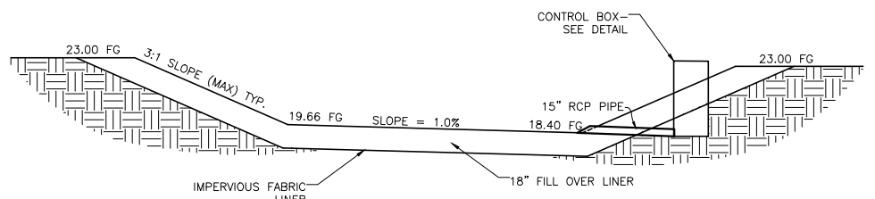
Detention Basin SCALE: NO SCALE
