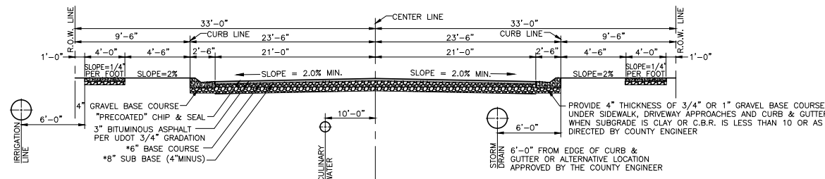
Street Section (66' R.O.W.) SCALE: NONE
