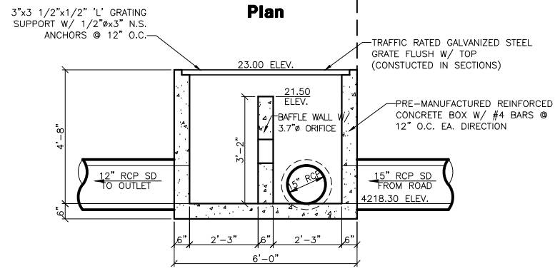
Detention Basin Control Box SCALE: 1" = 2"
