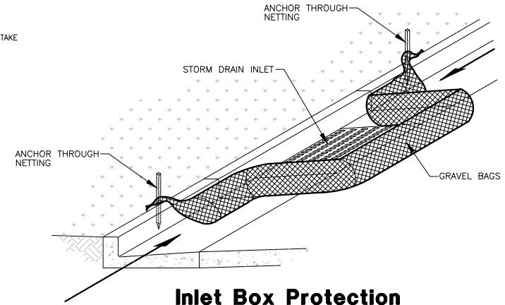
Inlet Box Protection
