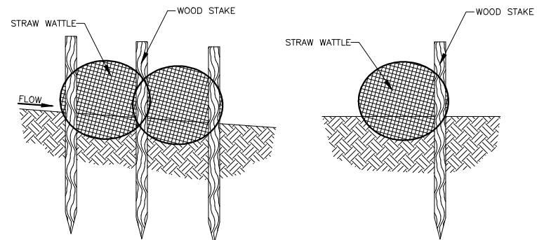
Stake Detail
