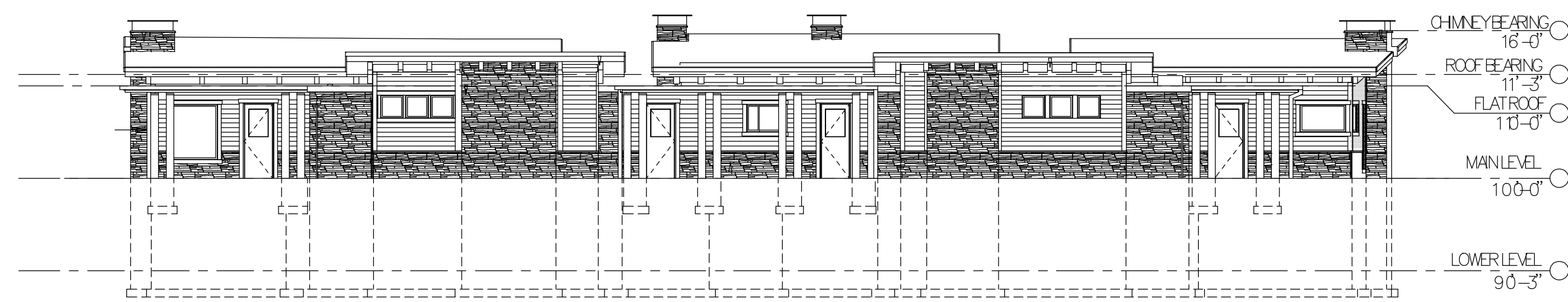
NORTH ELEVATION BUILDINGS 301-304 100'-00" = 5242.50 BUILDINGS 401-404 100'-00" = 5245.00
