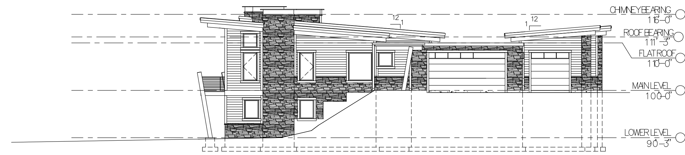
EAST ELEVATION BUILDINGS 301-304 100'-00" = 5242.50 BUILDINGS 401-404 100'-00" = 5245.00
