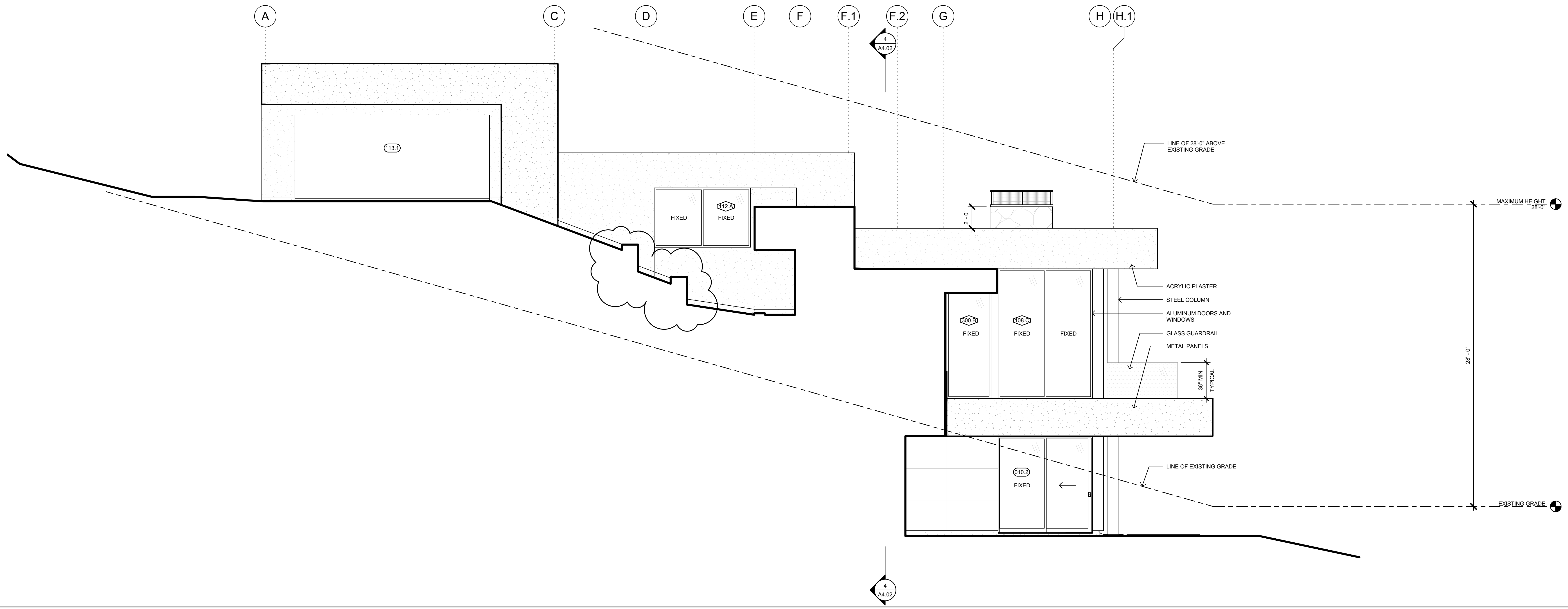
EXTERIOR ELEVATION - COURTYARD - EAST 1/4" = 1'-0" 2
