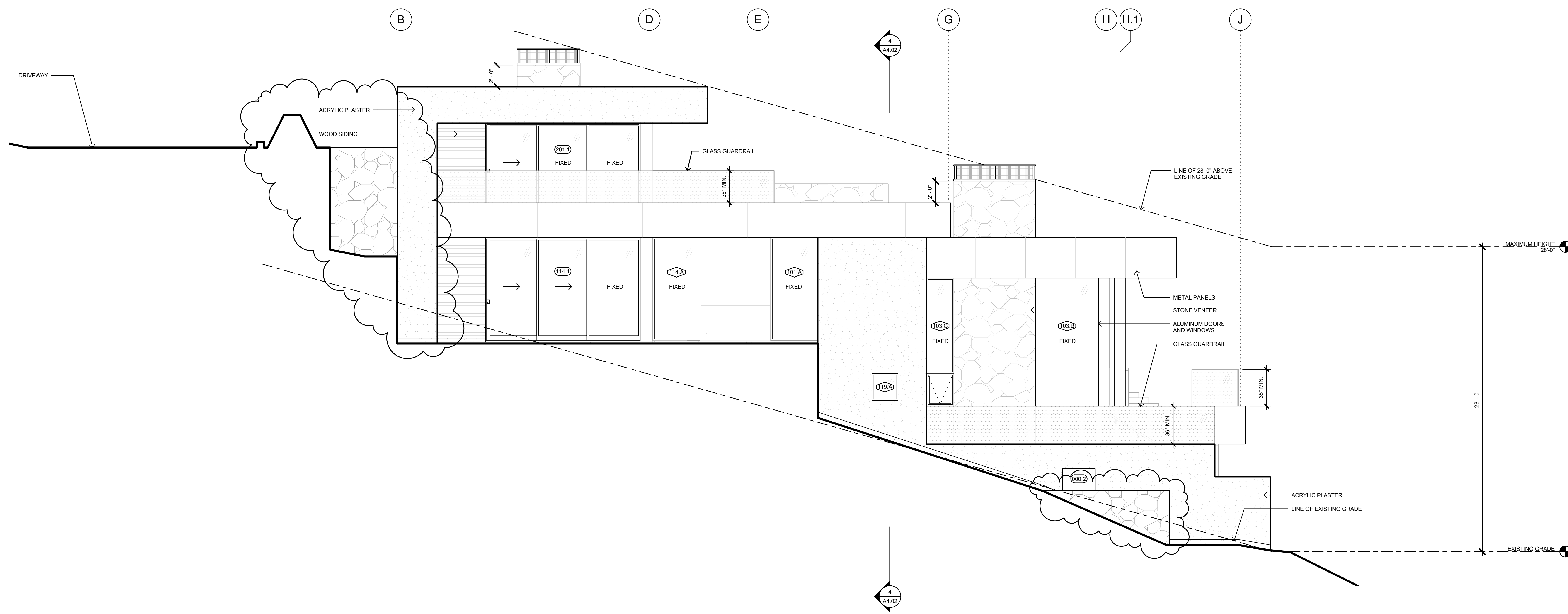
EXTERIOR ELEVATION - WEST 1/4" = 1'-0" 4
