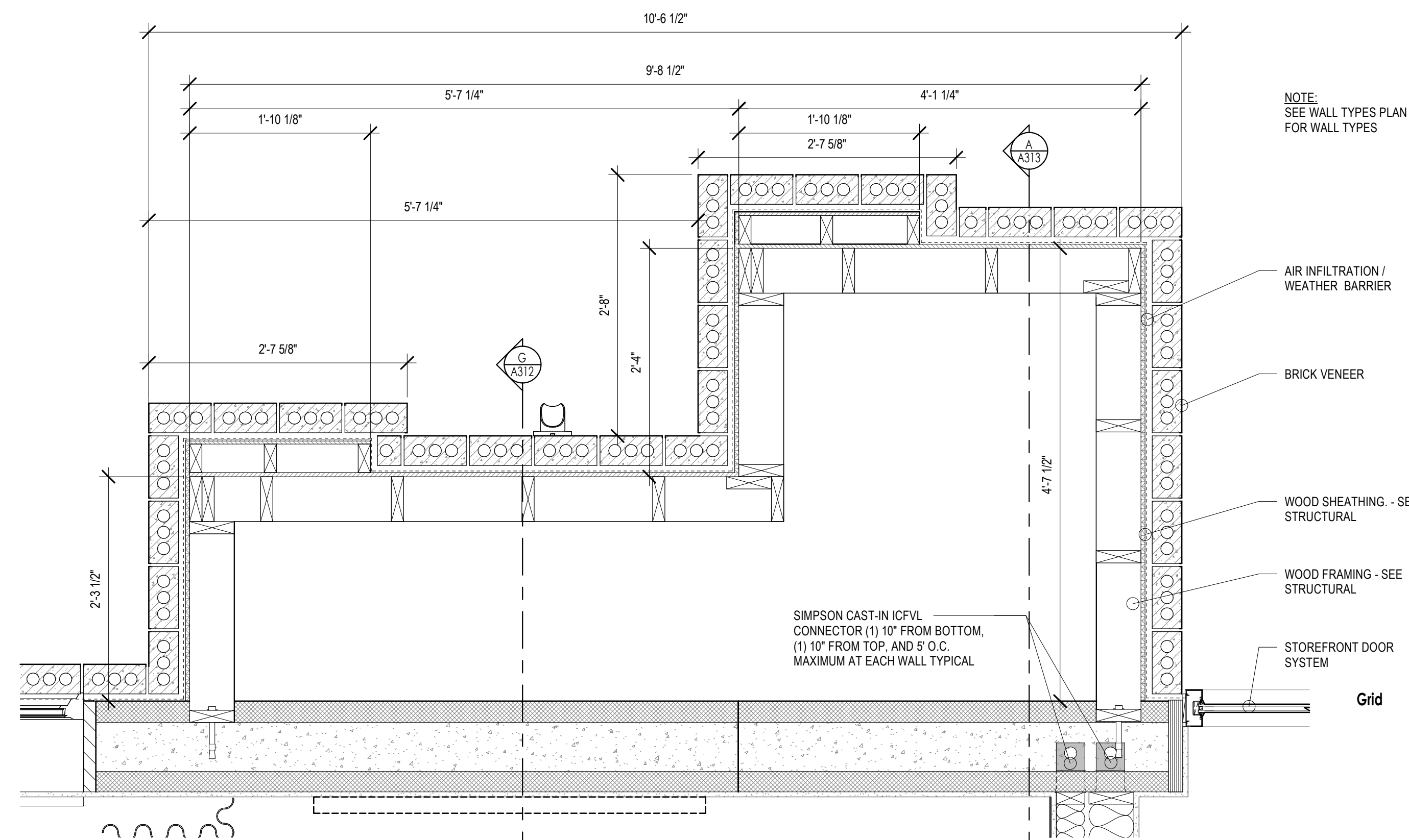
PILASTER DETAIL
