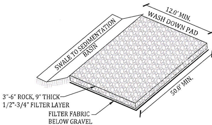
D TEMPORARY VEHICLE WASHDOWN & STABILIZED CONSTRUCTION ENTRANCE SCALE: NONE
