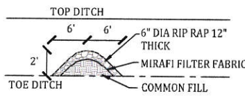
B-B' SECTION
