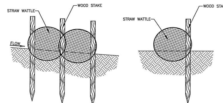
Stake Detail
