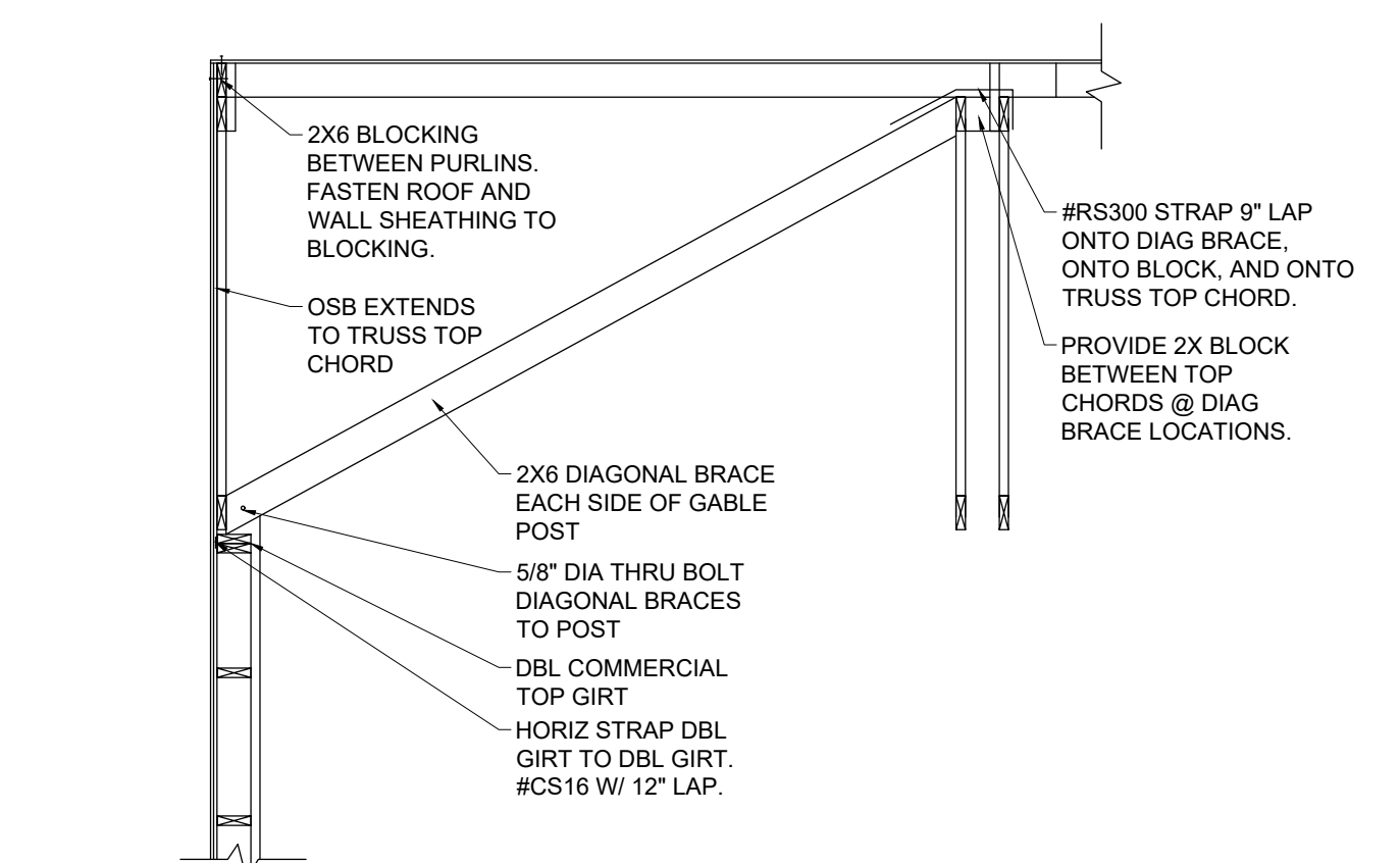
4 DIAGONAL BRACE A8 NTS
