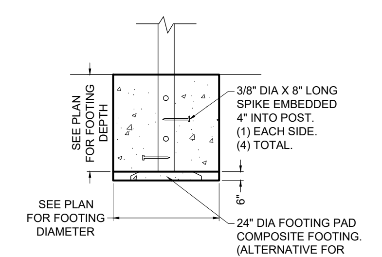
6 36"-42" DIA FOOTING A8 NTS
