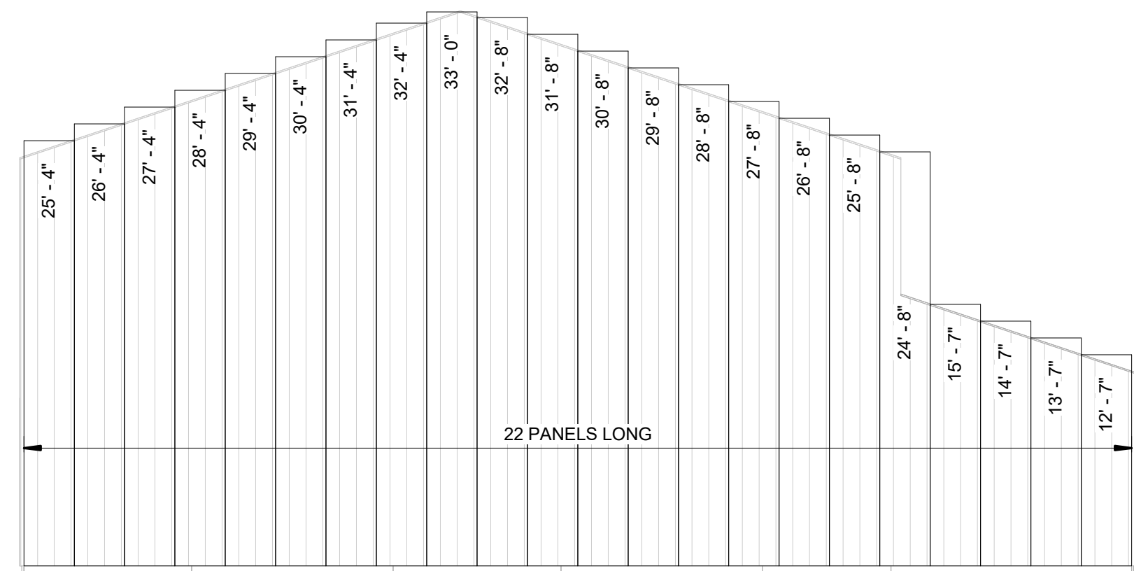
3 SOUTH PANEL 1/8" = 1'-0"
