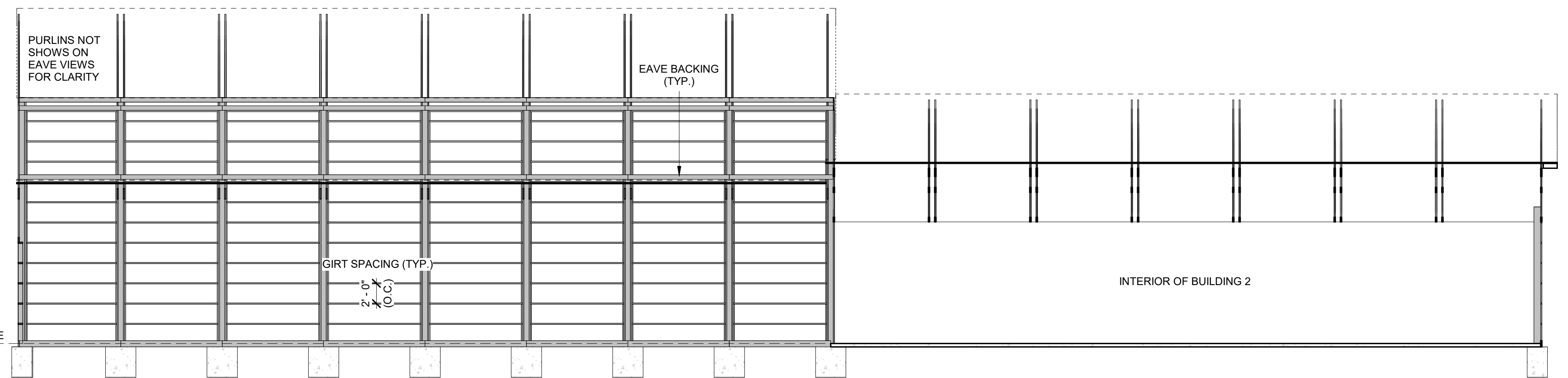
6 EAST GIRT (BUILDING 1) 1/8" = 1'-0"
