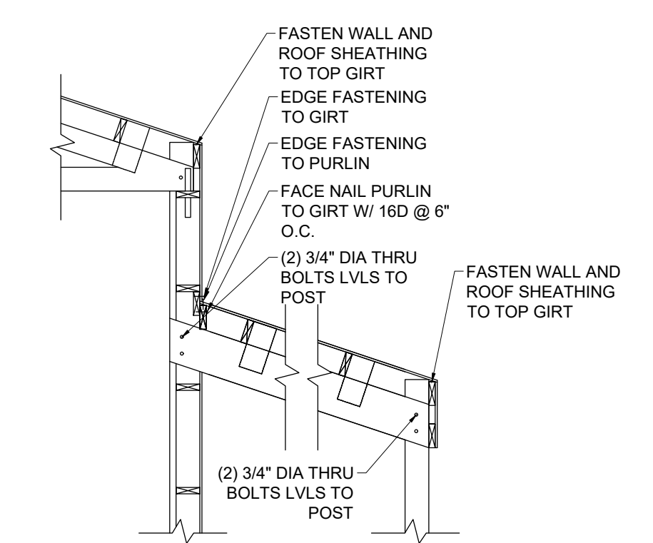
11 OFFSET LEAN SECTION A8 NTS
