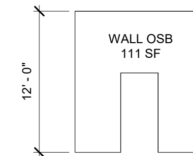
15 NORTH OSB (TOILET ROOM) 1/8" = 1'-0"
