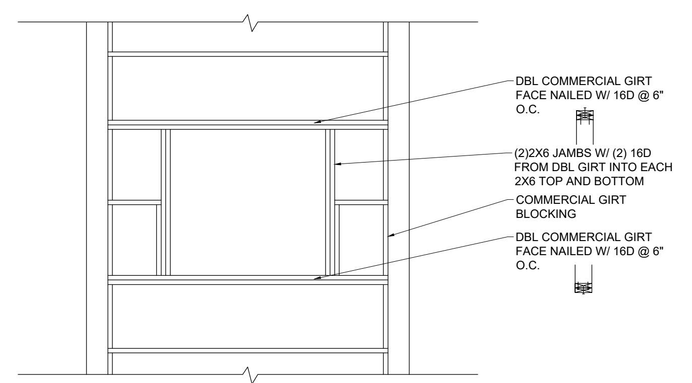
12 WINDOW FRAMING A8 NTS
