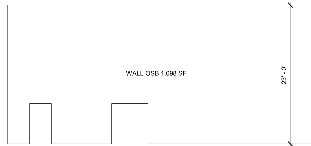
3 SOUTH OSB (BUILDING 1) 1/8" = 1'-0"
