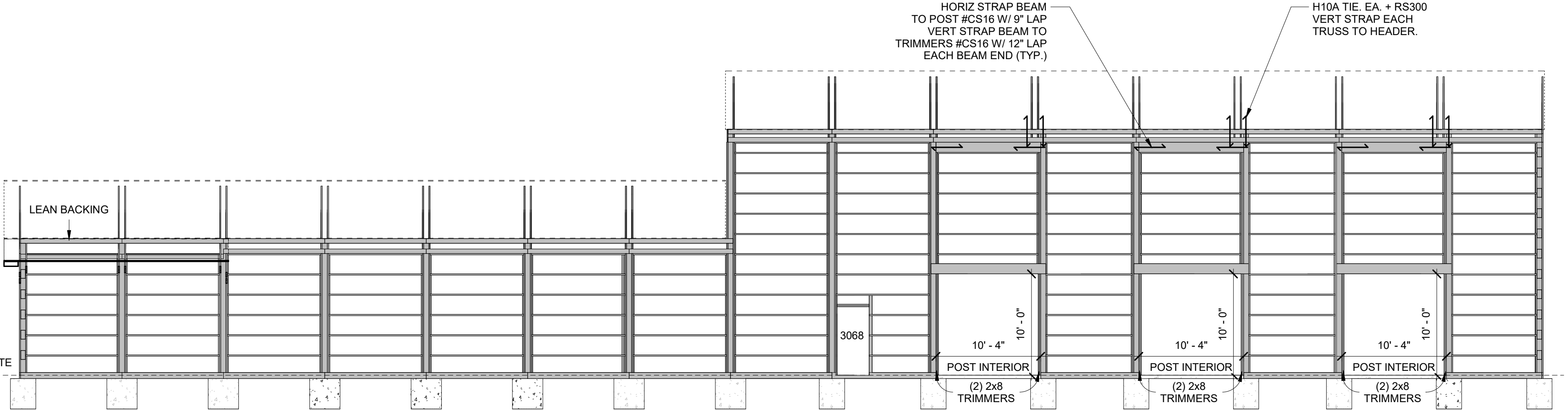
4 WEST GIRT 1/8" = 1'-0"
