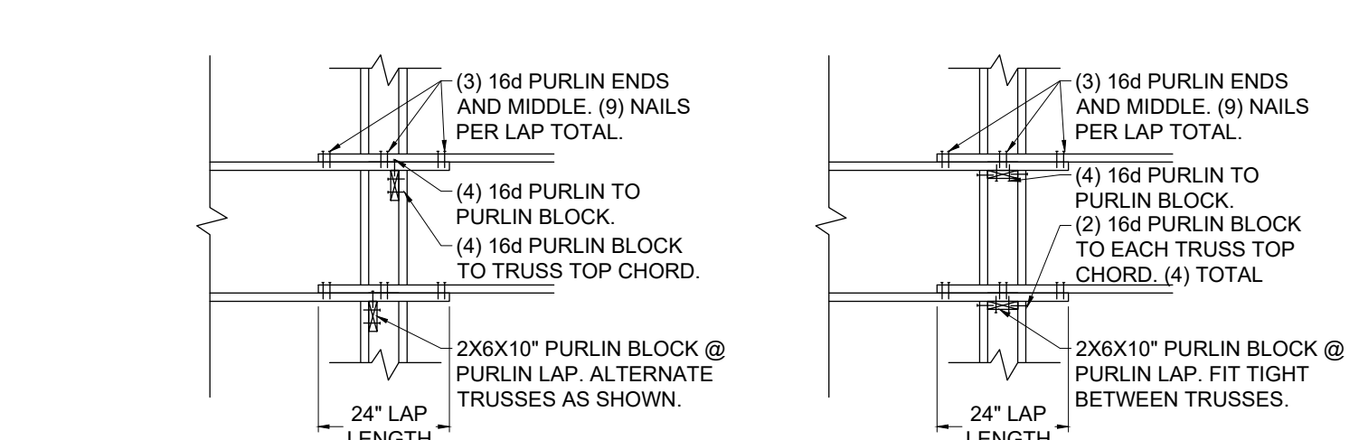
3 PURLIN LAP -OR- PURLIN LAP A8 NTS
