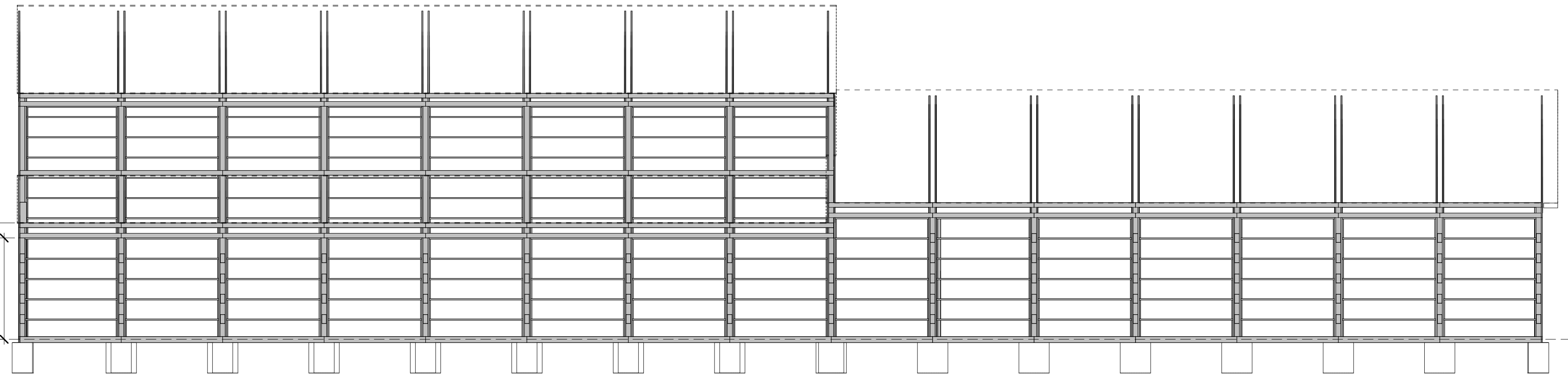
2 EAST GIRT (BUILDING 2 & LEAN) 1/8" = 1'-0"
