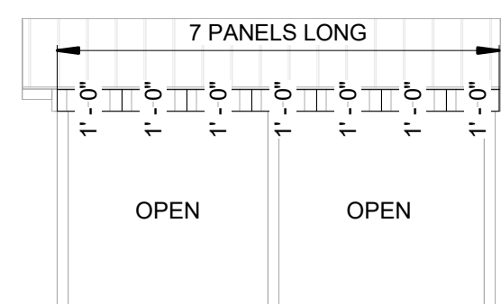
5 WEST PANEL (LEAN) 1/8" = 1'-0"
