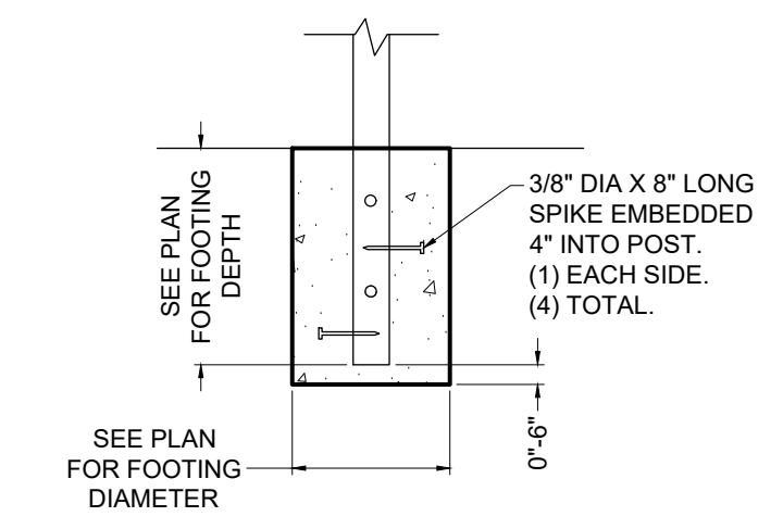
1 24"-30" DIA FOOTING A8 NTS
