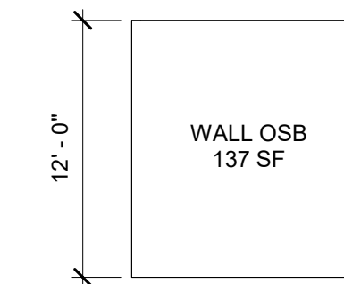
17 SOUTH OSB (TOILET ROOM) 1/8" = 1'-0"
