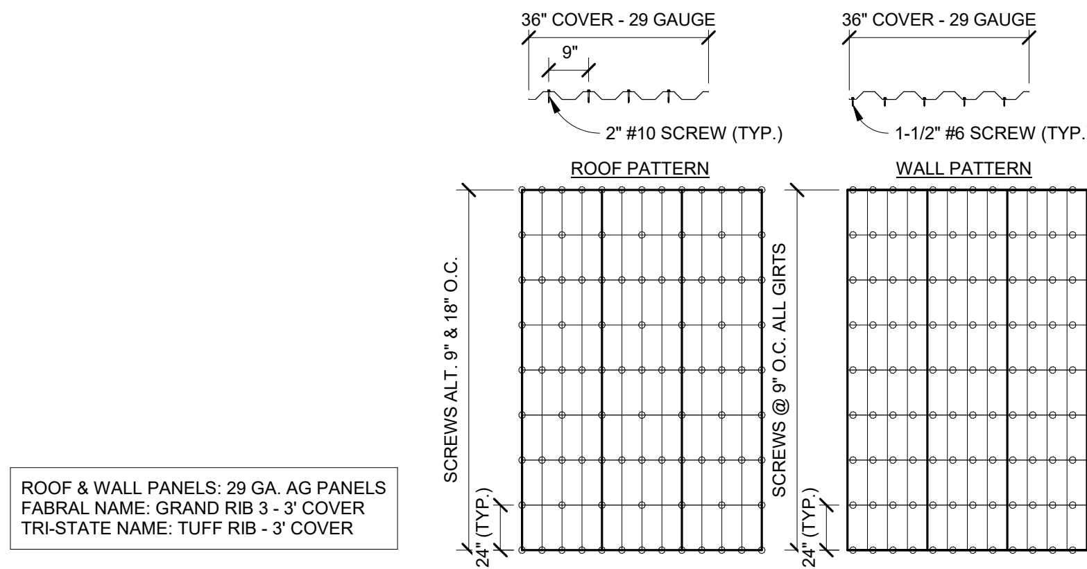
⑥ ROPER BUILDINGS SCREW PATTERNS 1" = 10'-0"
