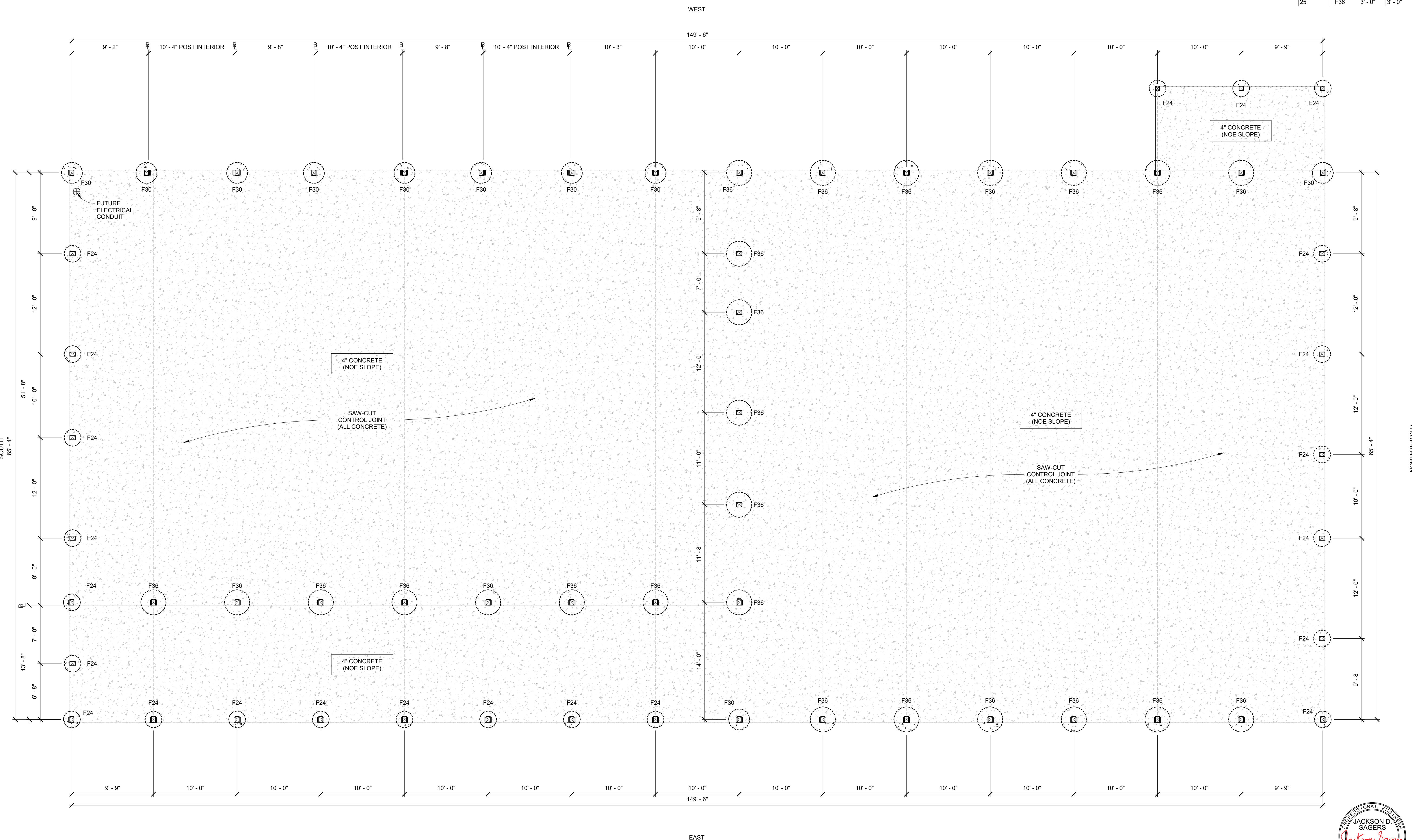
FOUNDATION PLAN 3/16" = 1'-0"
