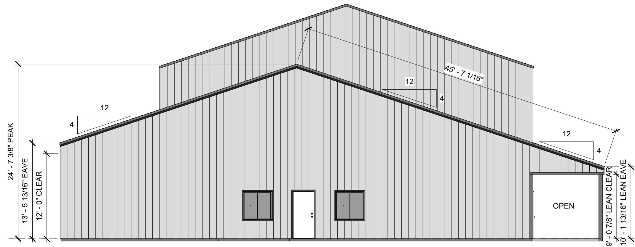
① NORTH (FRONT) ELEVATION 1/8" = 1'-0"
