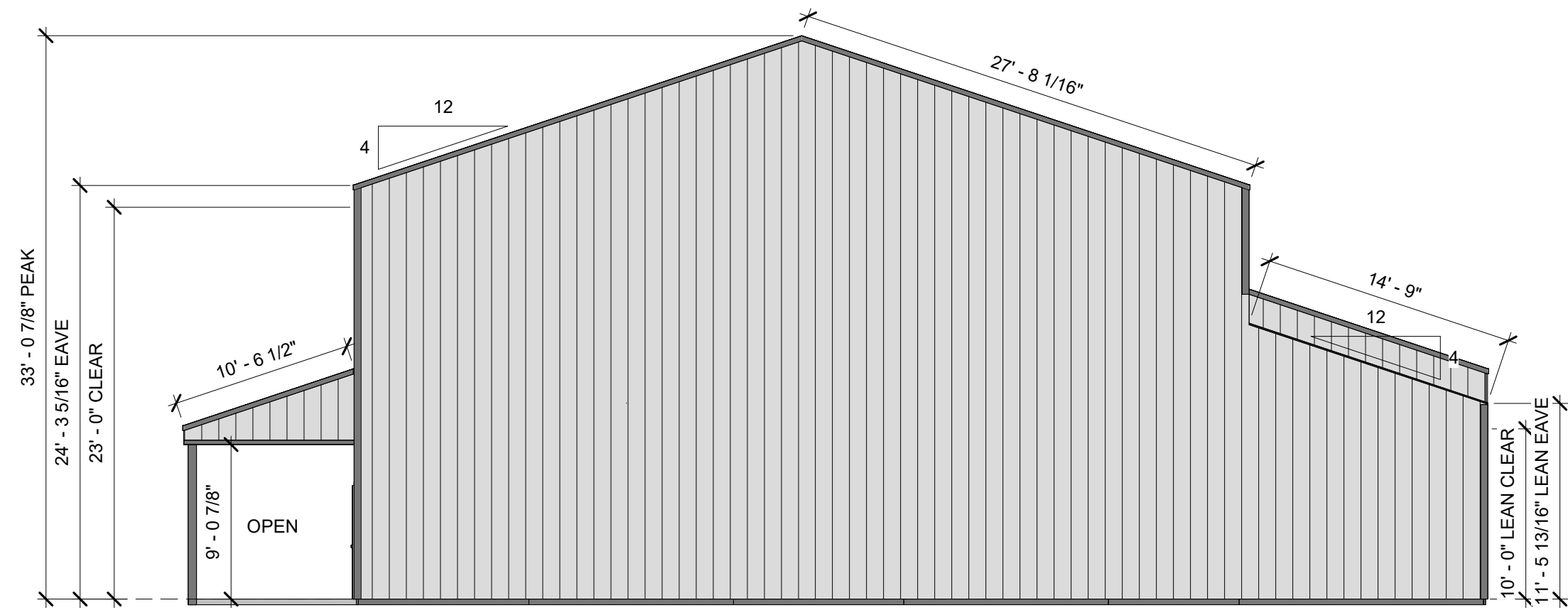
③ SOUTH ELEVATION 1/8" = 1'-0"
