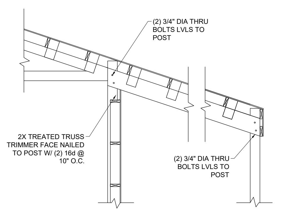
10 LVL TO TRUSS LEAN SECTION A8 NTS
