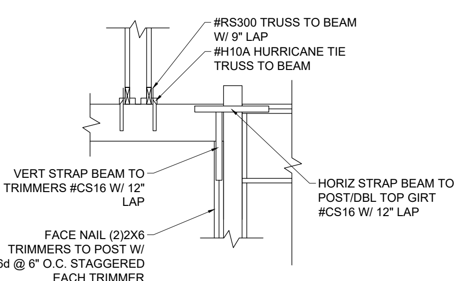
14 BEARING GARAGE HDR A8 NTS
