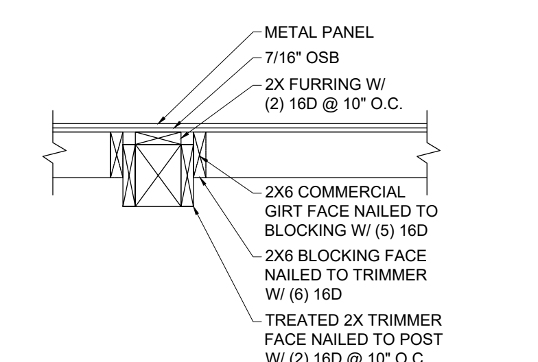
7 SECTION AT POST A8 NTS
