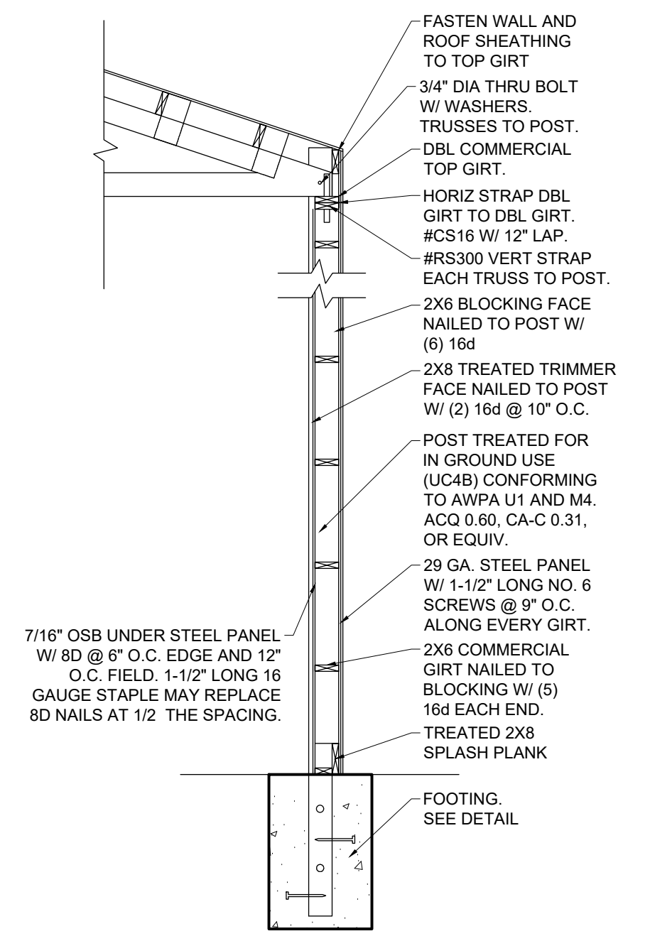
5 WALL SECTION A8 NTS
