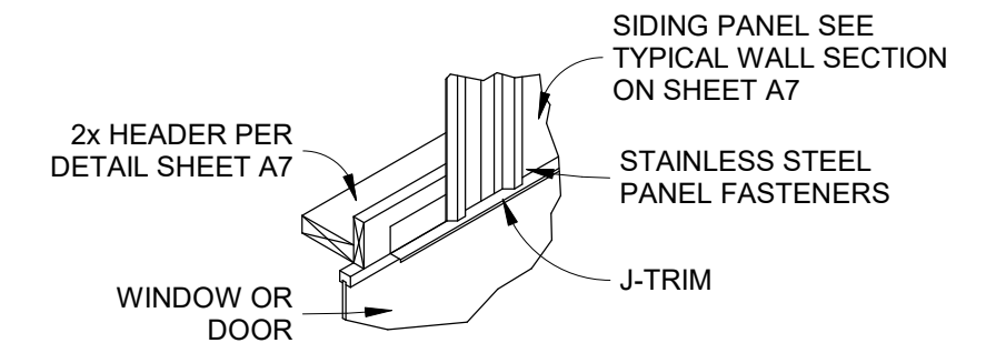
④ WINDOW/DOOR HEADER FLASHING N.T.S.
