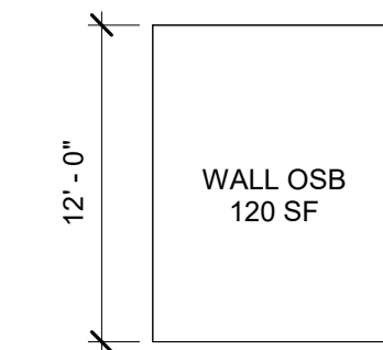
16 EAST OSB (TOILET ROOM) 1/8" = 1'-0"
