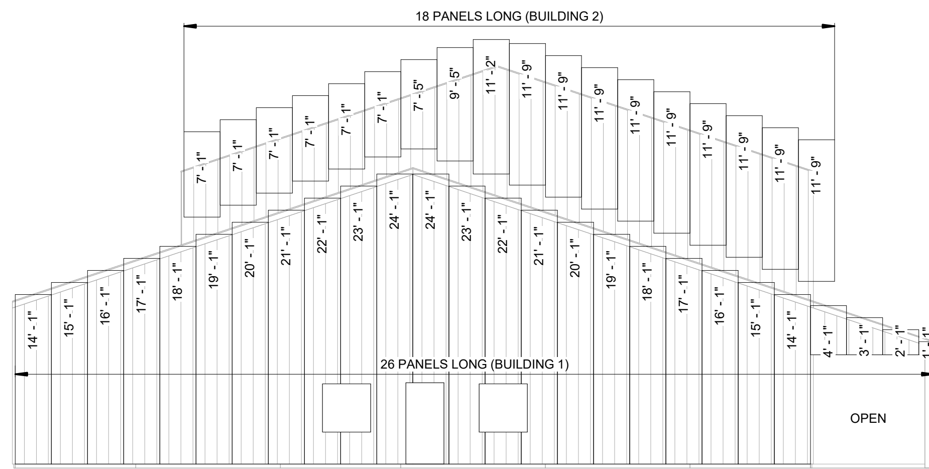
1 NORTH PANEL 1/8" = 1'-0"
