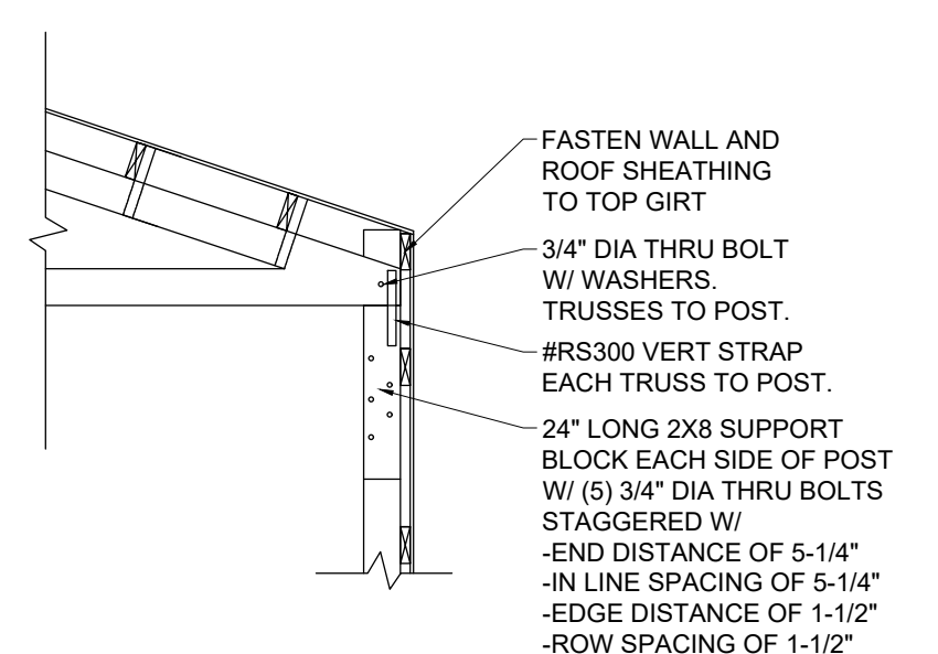
9 3/4" THRU BOLT TRUSS SUPPORT ALTERNATIVE A8 NTS
