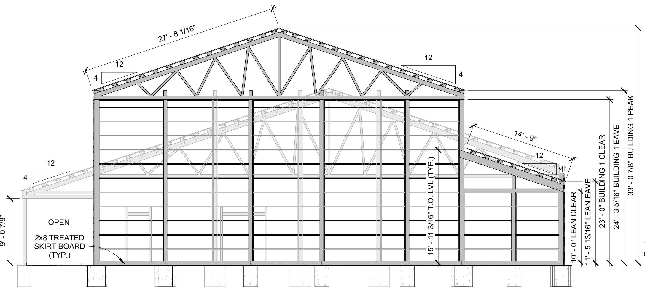
3 SOUTH GIRT 1/8" = 1'-0"
