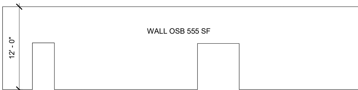
9 SOUTH OSB (BUILDING 2) 1/8" = 1'-0"
