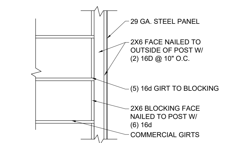
2 CORNER BLOCKING A8 NTS
