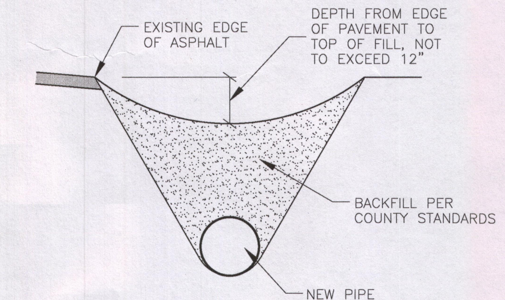
Pipe/Ditch Backfill Detail
