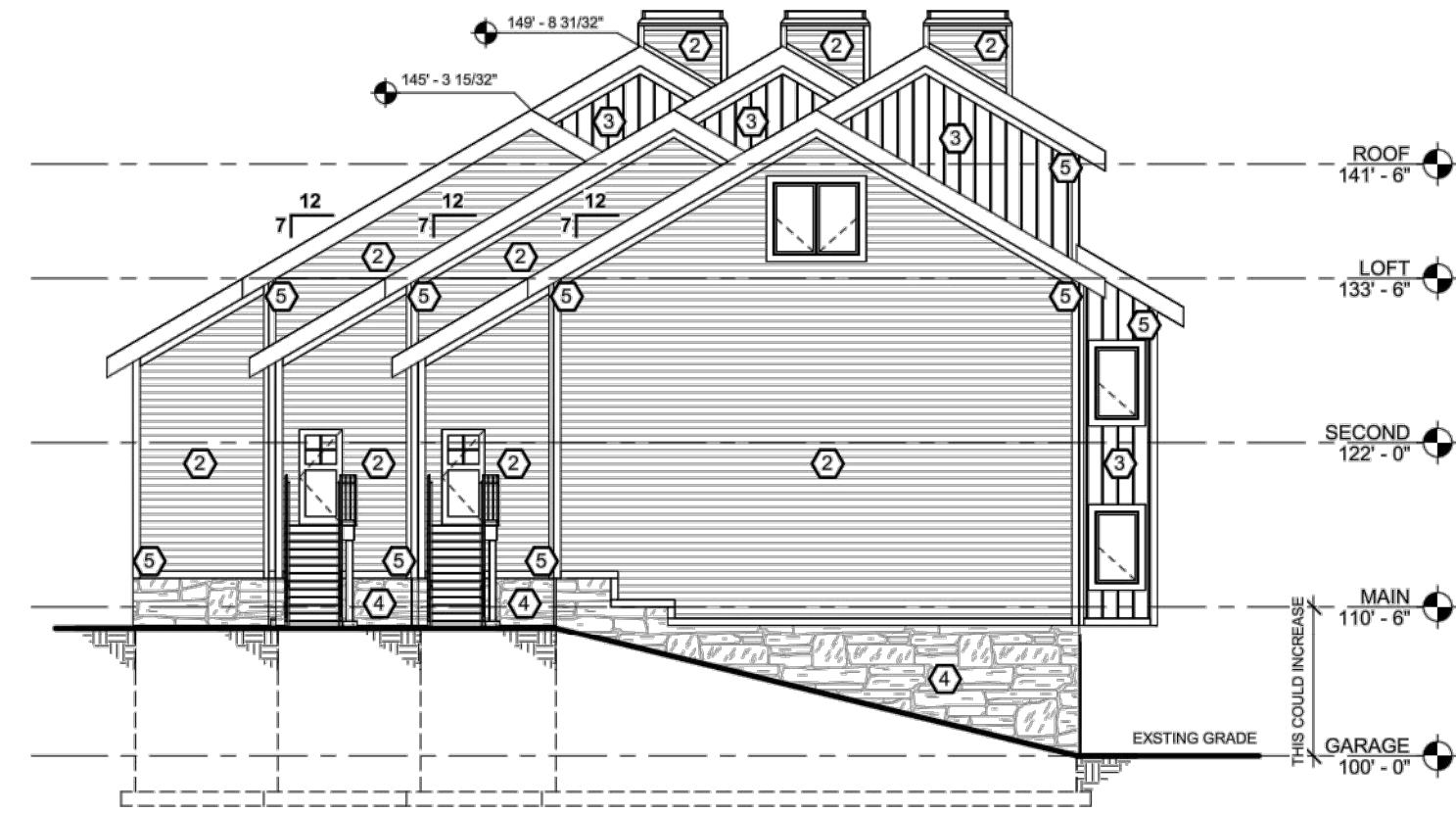
LEFT ELEVATION
