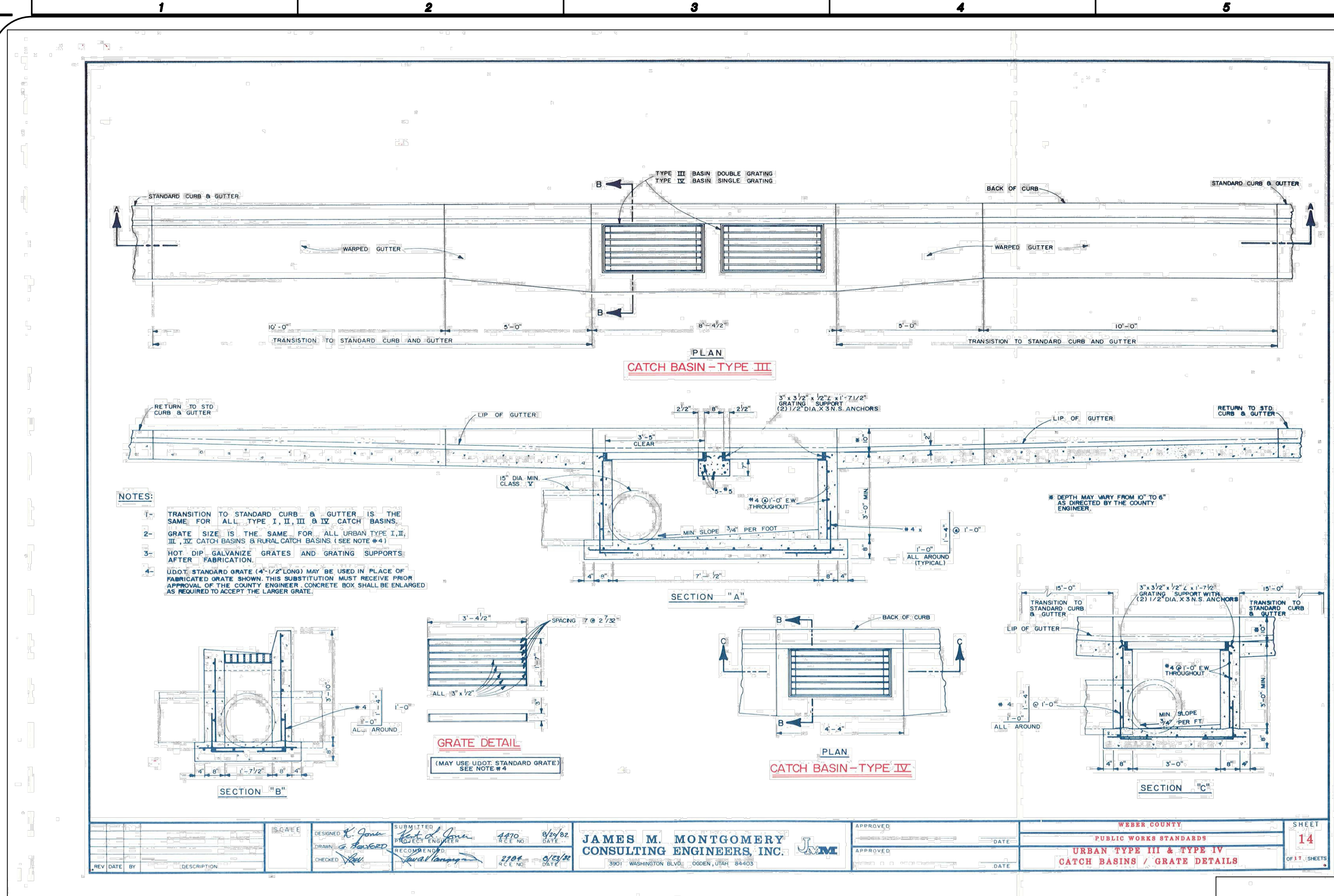
A Typical Catch Basin Details SW2 Not to Scale
