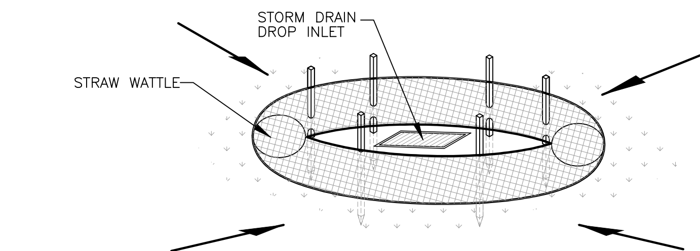
Drop Inlet Protection
