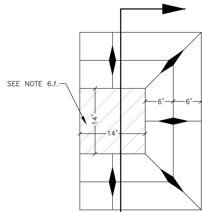
Concrete Washout Area w/ 10 mil Plastic Liner
