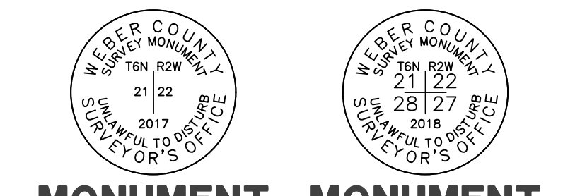
MONUMENT DETAIL 3 (NOT TO SCALE) MONUMENT DETAIL 4 (NOT TO SCALE)
