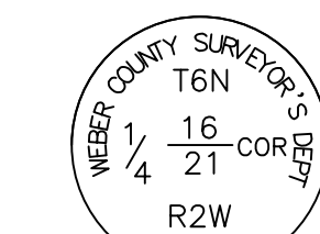
MONUMENT DETAIL 2 (NOT TO SCALE)
