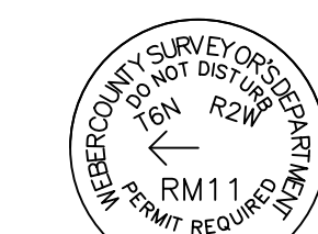
MONUMENT DETAIL 5 (NOT TO SCALE)
