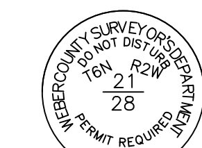
MONUMENT DETAIL 4 (NOT TO SCALE)
