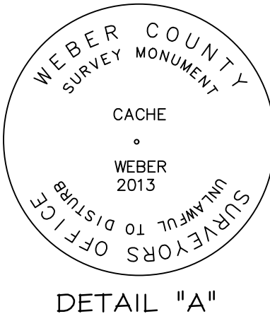
DETAIL "A"
