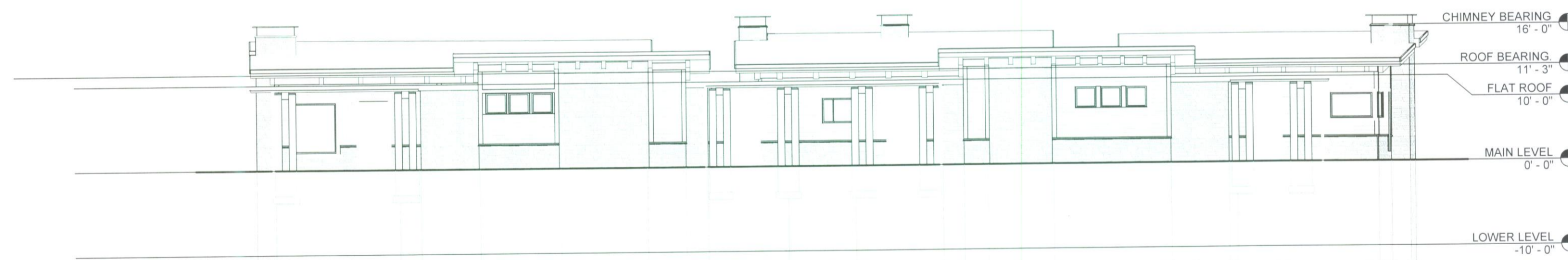
NORTH ELEVATION BUILDINGS 1-4 100'-00" = 5218.70 BUILDINGS 5-8 100'-00" = 5220.00
