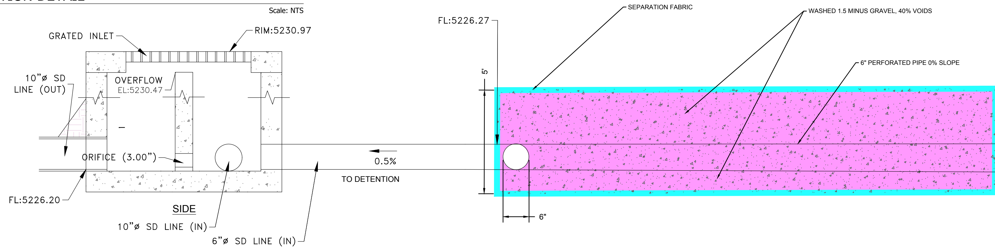
14 DETENTION DETAIL
