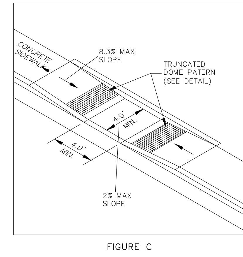
5 TYPICAL ADA RAMP Scale: NTS
