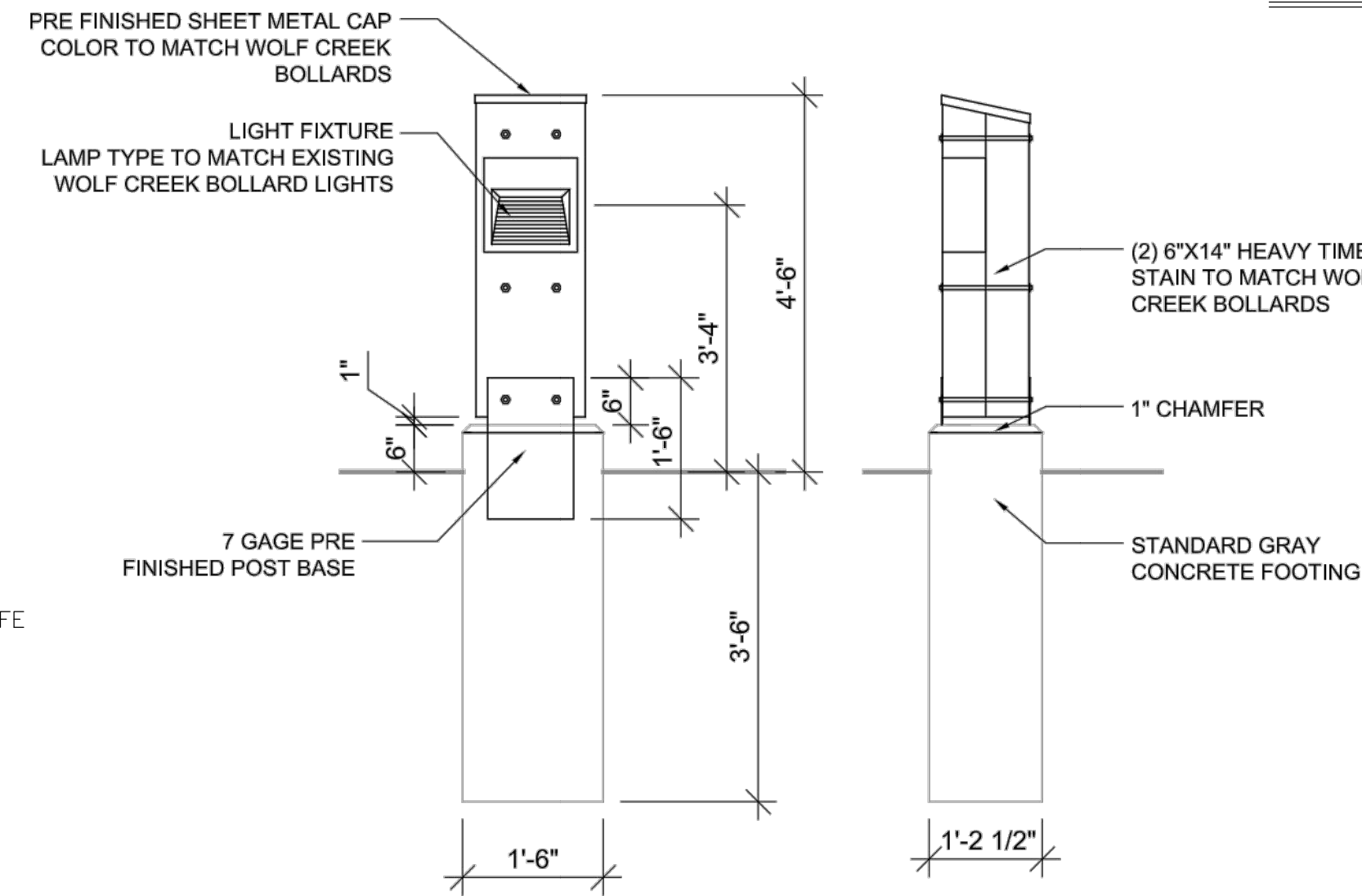
12 BOLLARD LIGHT
