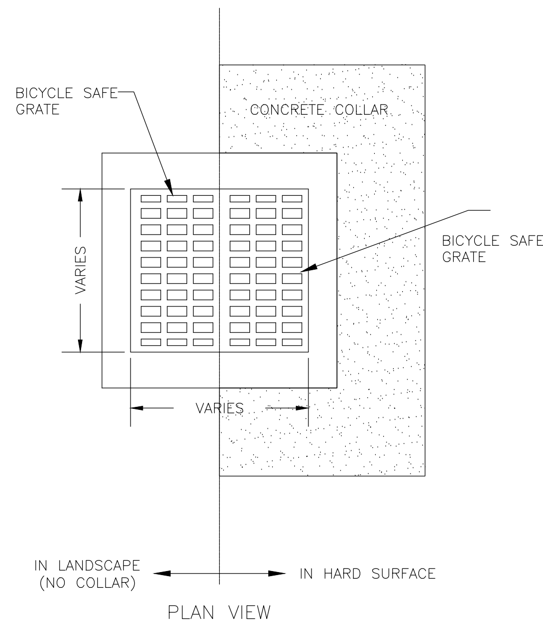
TYPICAL STORM DRAIN BOX
