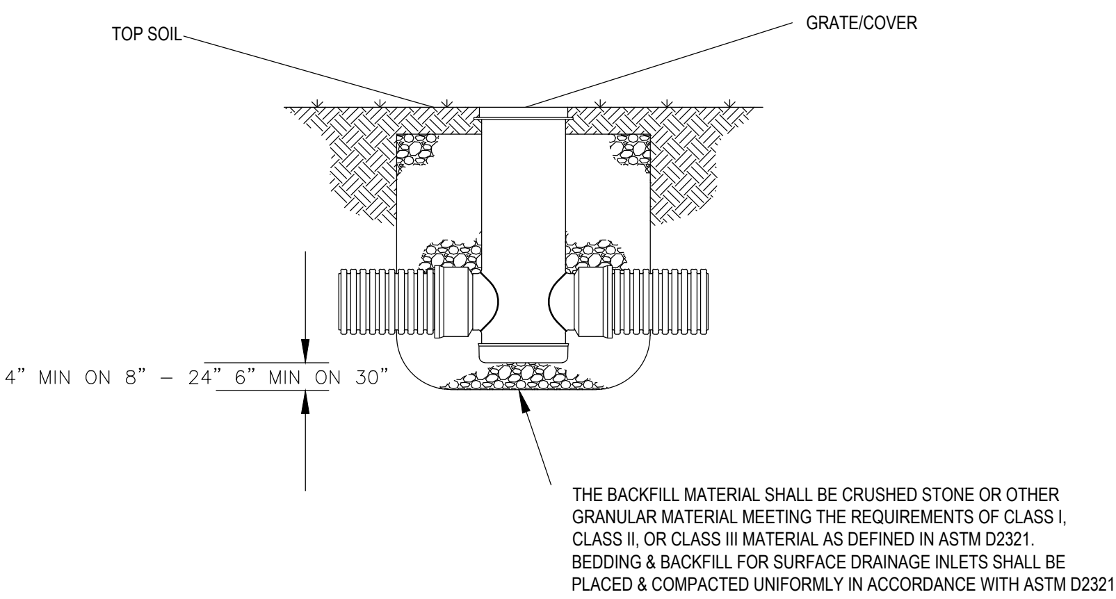
10 TYPICAL STORM DRAIN BOX
