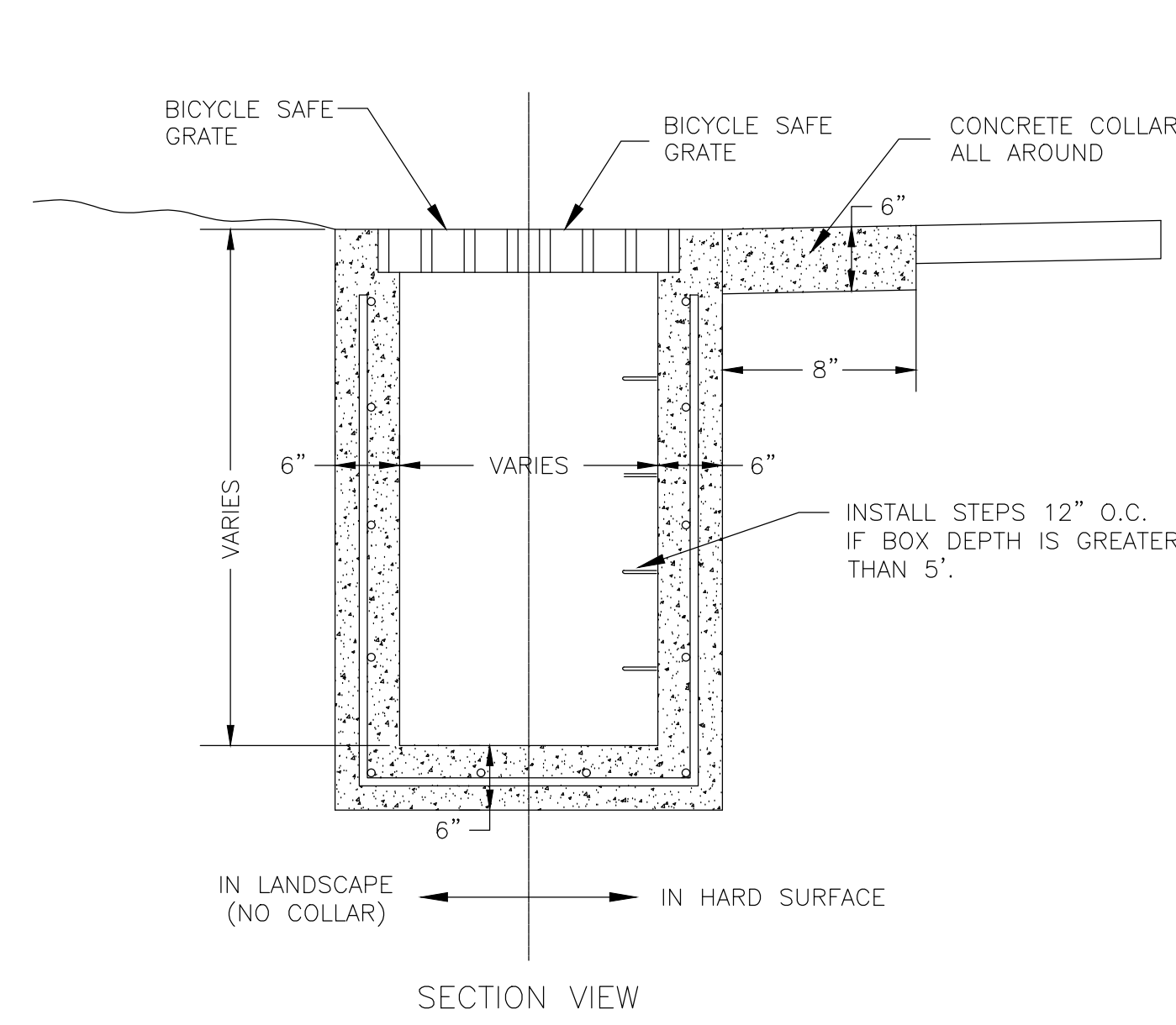
TYPICAL STORM DRAIN BOX
