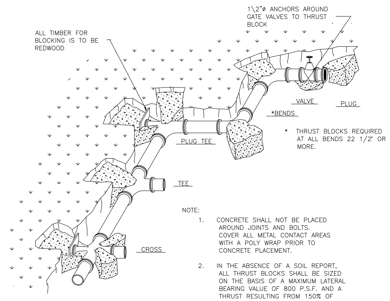
4 TYPICAL THRUST BLOCK DETAIL APPLIES TO ALL PRESSURE PIPE Scale: NTS
