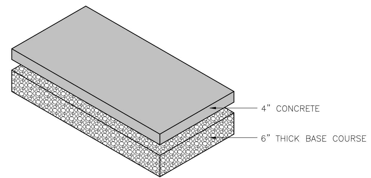
6 CONCRETE SIDEWALK SECTION Scale: NTS
