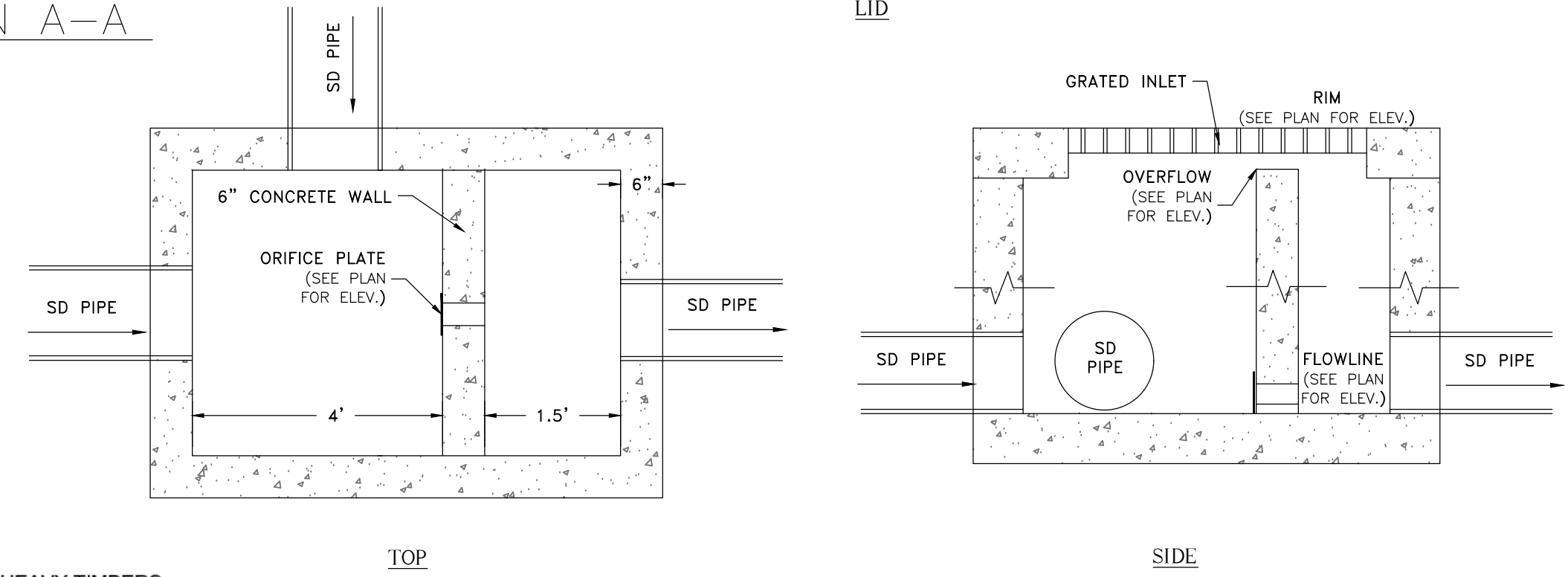
CONTROL STRUCTURE DETAIL
