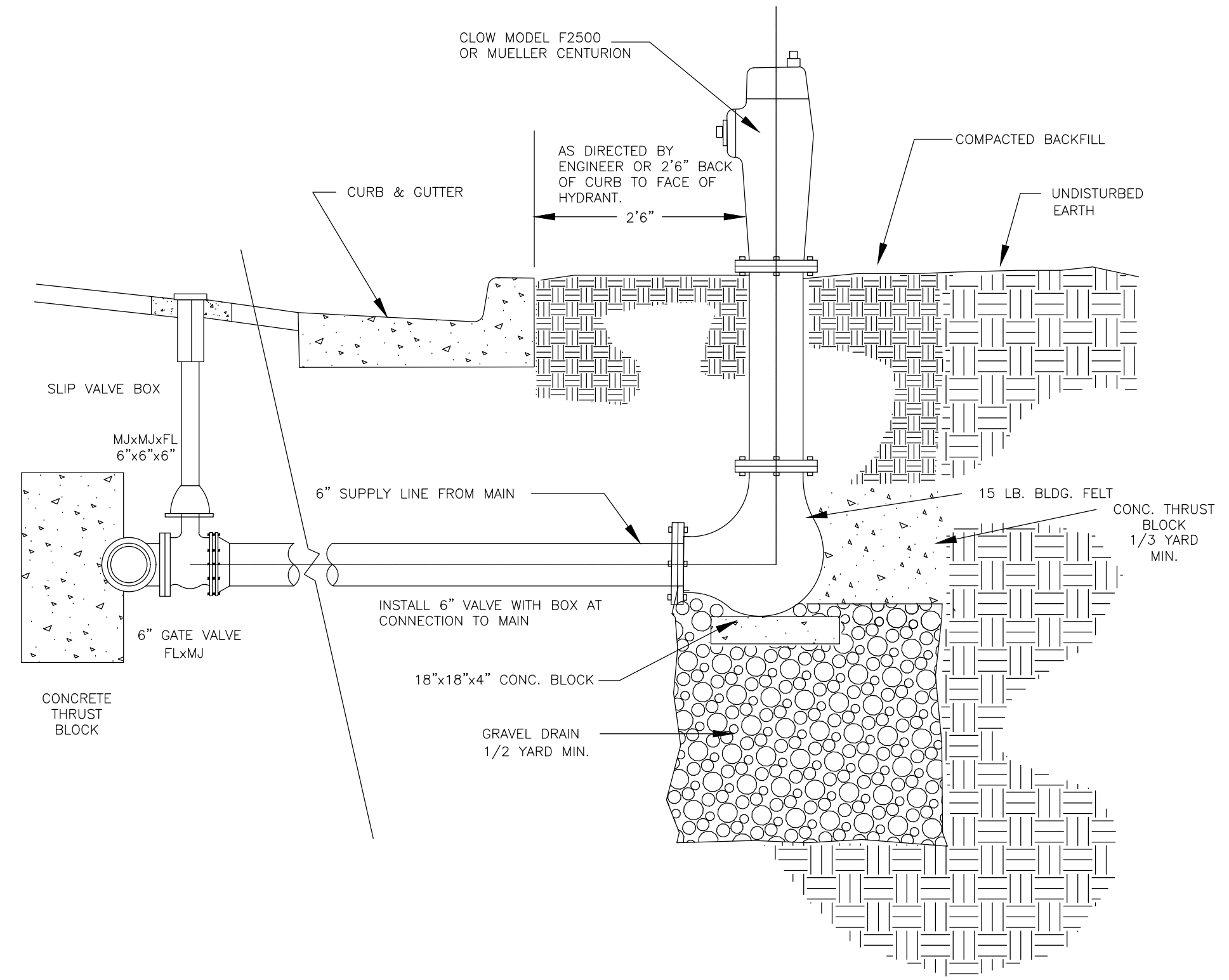
3 TYPICAL WATER HYDRANT INSTALLATION DETAIL Scale: NTS
