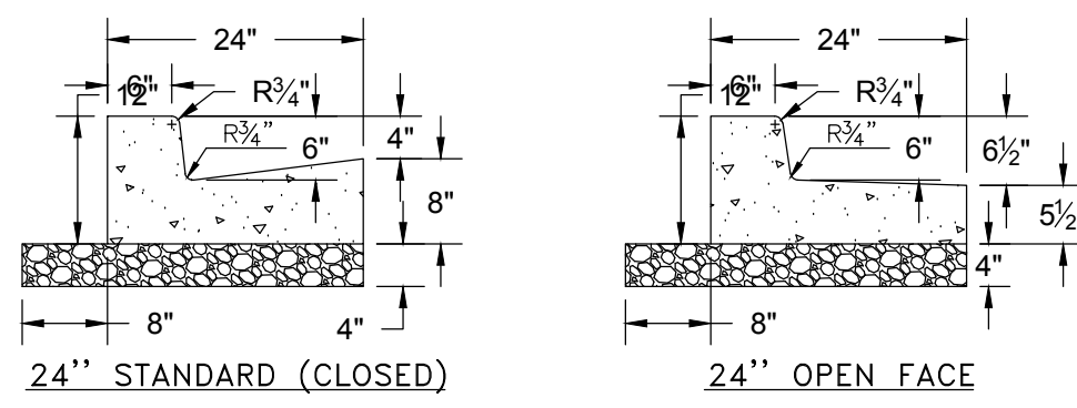
TYPICAL 24' CURB AND GUTTER NOT TO SCALE
