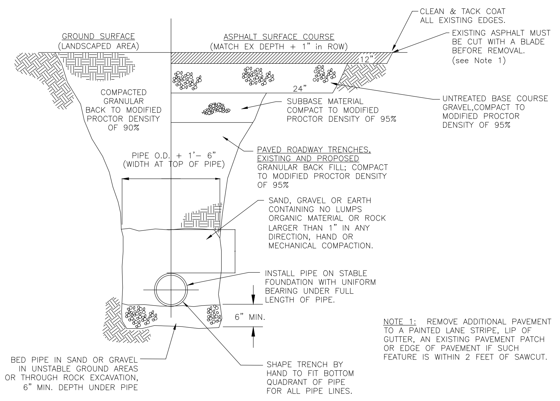
2 TYPICAL TRENCH SECTION Scale: NTS
