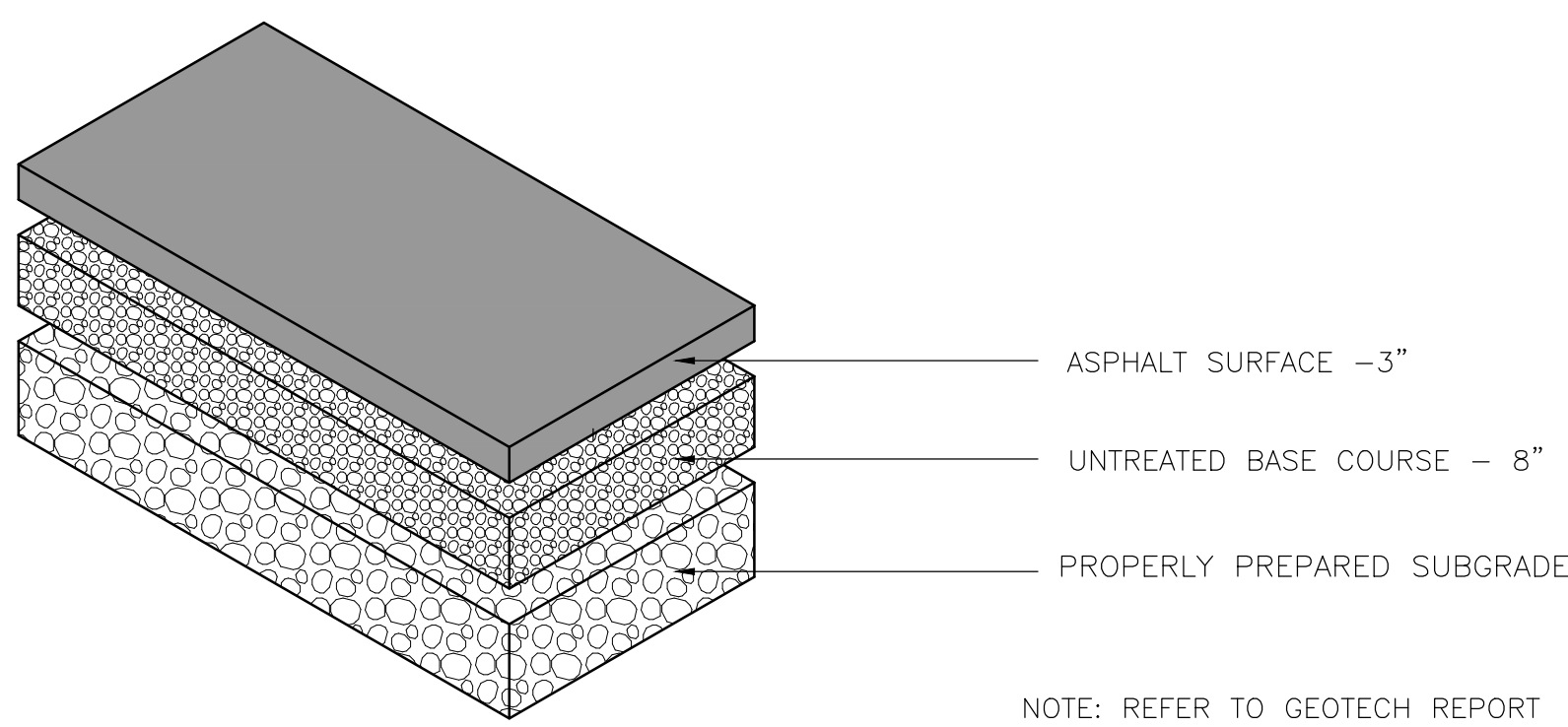
7 TYPICAL REGULAR ASPHALT PAVING Scale: NTS
