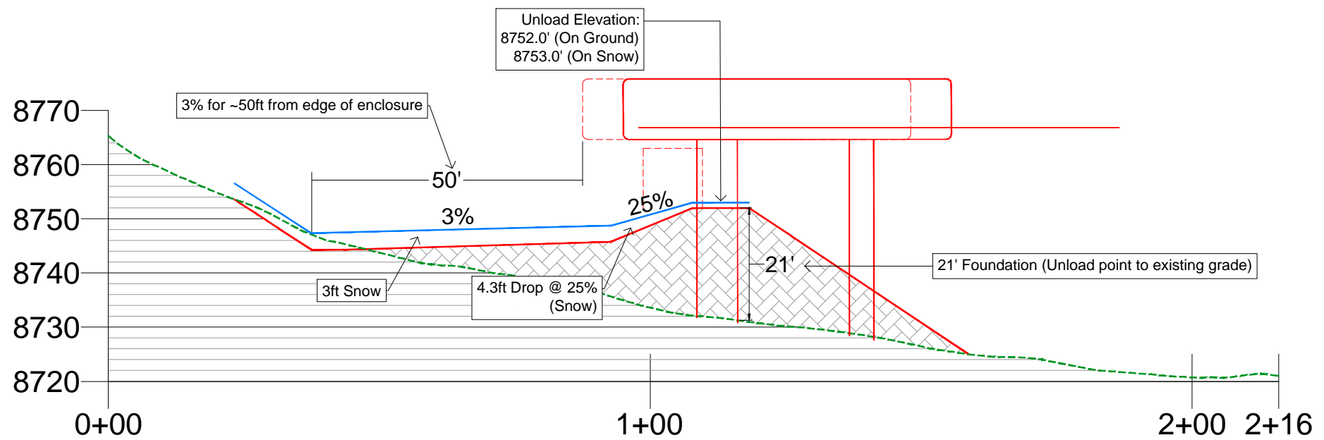
Middle Bowl Top Terminal - Grading Concept 3c - Profile
