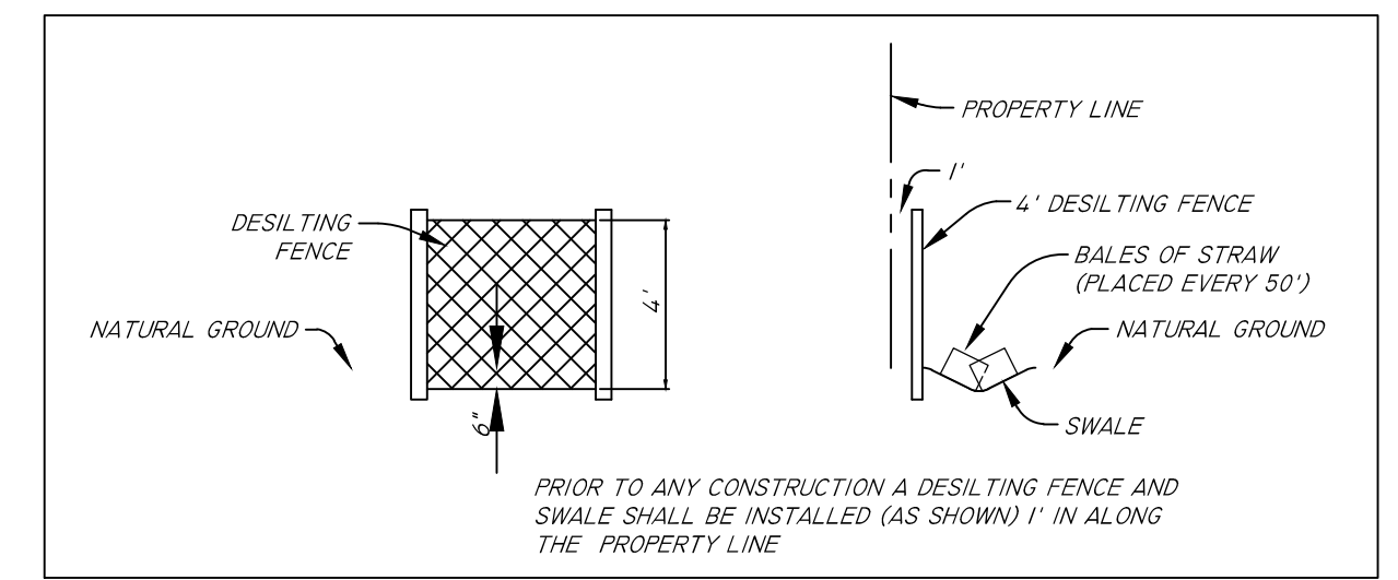
DESILTING FENCE DETAIL NOT TO SCALE
