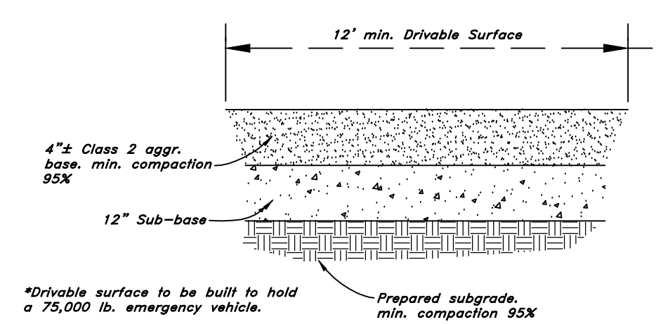
Gravel Drive Detail
