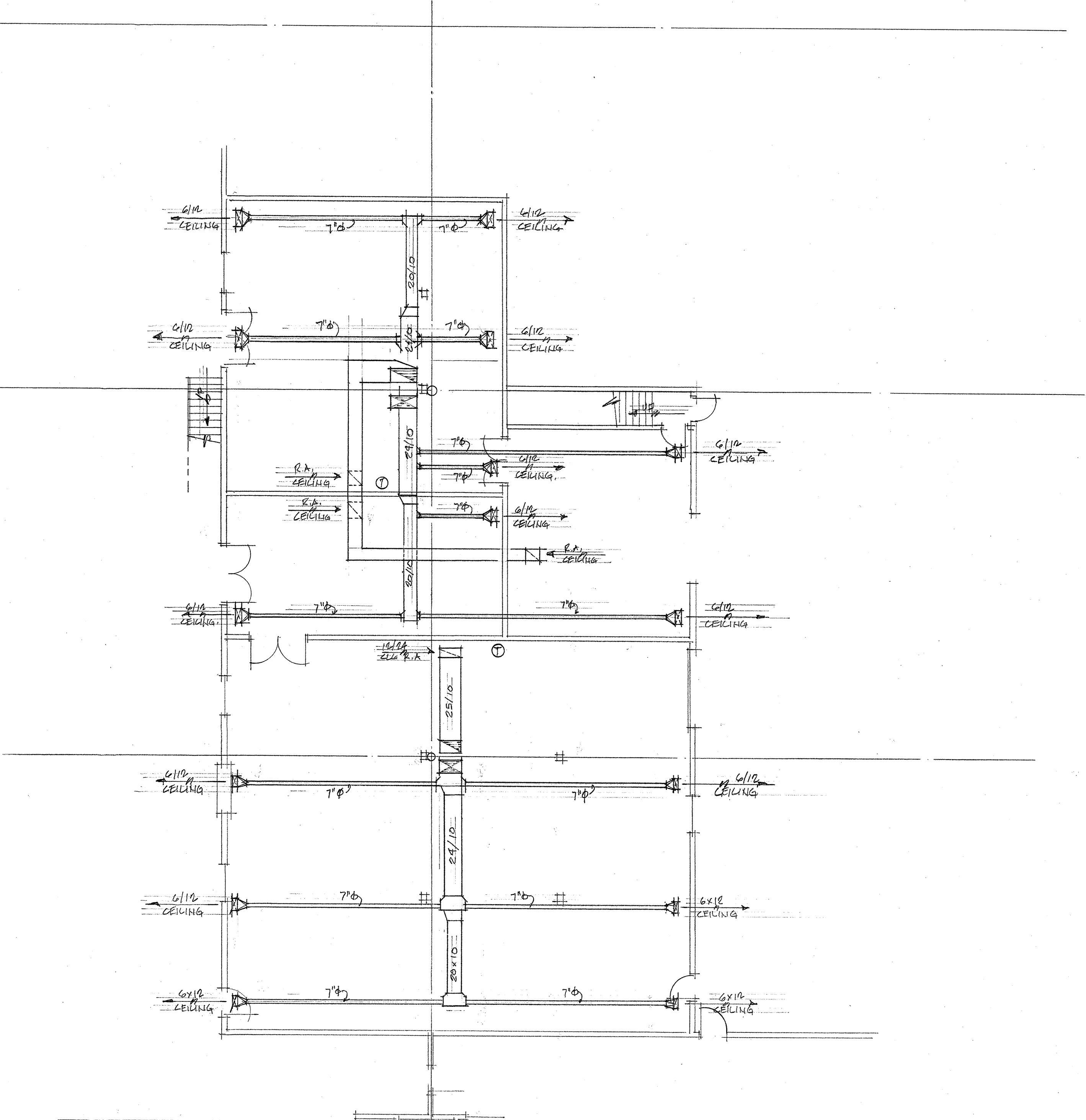
MAIN FLOOR MECHANICAL PLAN SCALE: 1/8" = 1'-0"
