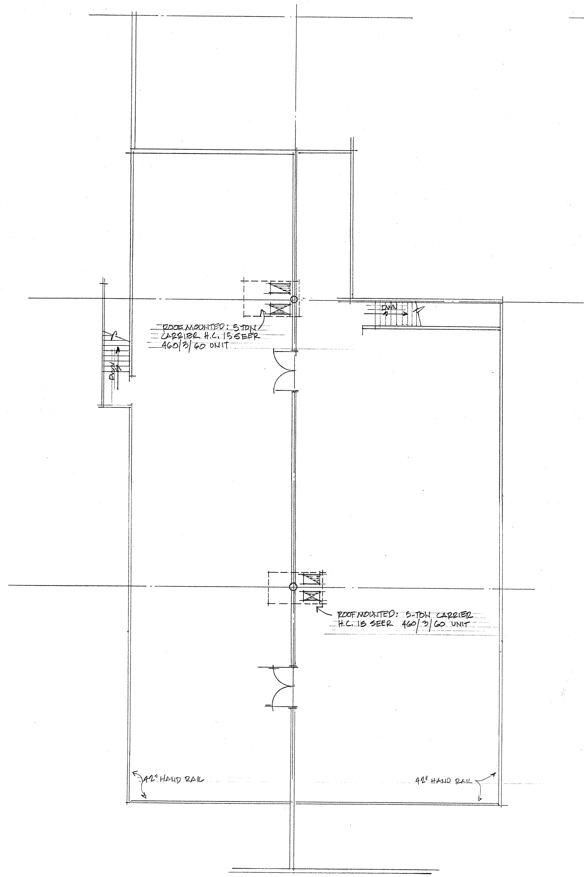
UPPER MEZZ MECHANICAL PLAN SCALE: 1/8" = 1'-0"
