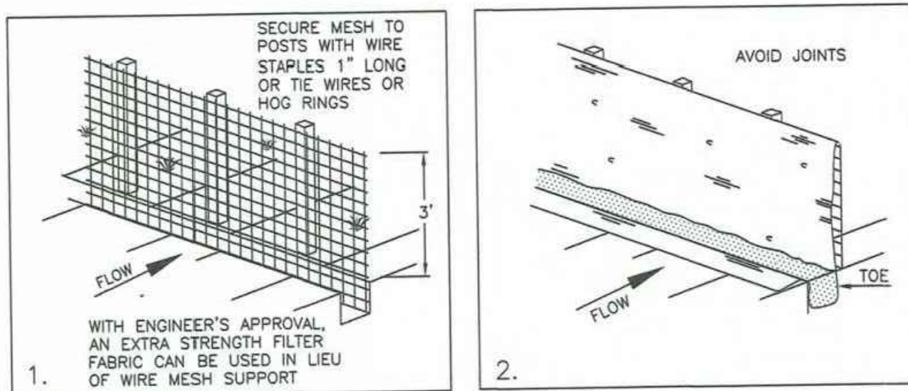
INSTALLATION SEQUENCE
