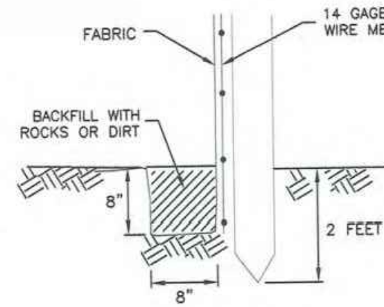
TOE DETAIL
